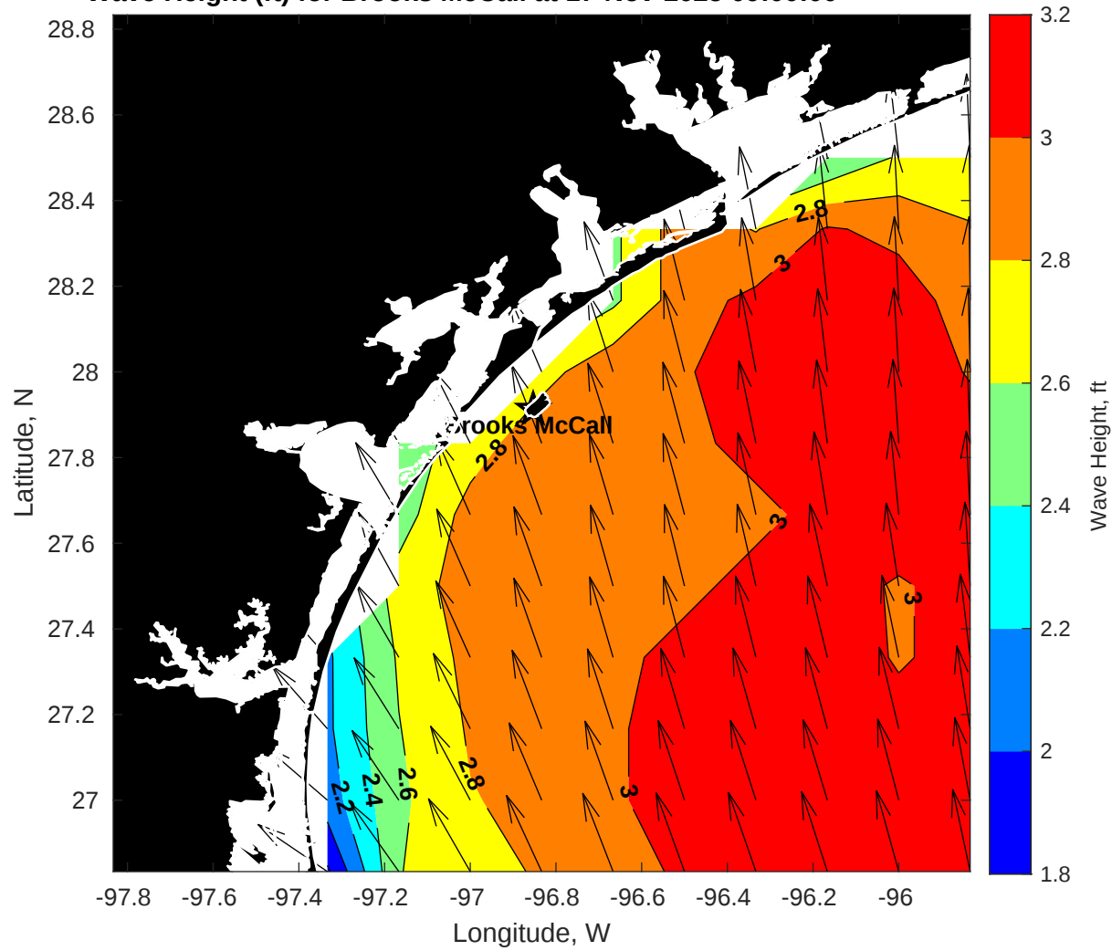
Wave Height (ft) for Brooks McCall at 17-Nov-2025 09:00:00
