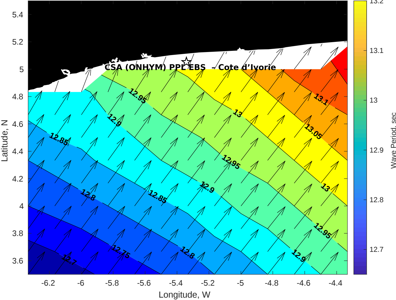
Wave Period (sec) for CSA (ONHYM) PPL EBS - Cote d'Ivoire at 17-Nov-2025 09:00:00
