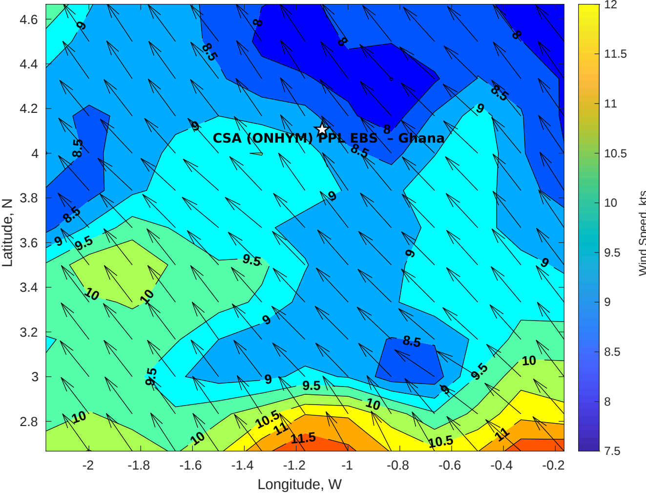
Winds (kts) for CSA (ONHYM) PPL EBS - Ghana at 17-Nov-2025 09:00:00
