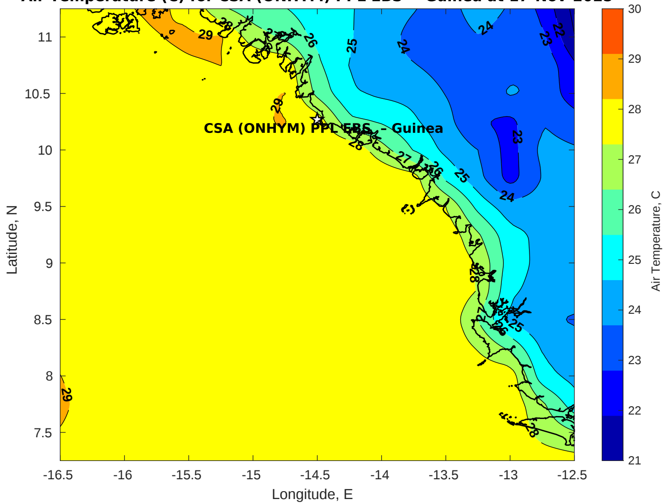
Air Temperature (C) for CSA (ONHYM) PPL EBS - Guinea at 17-Nov-2025
