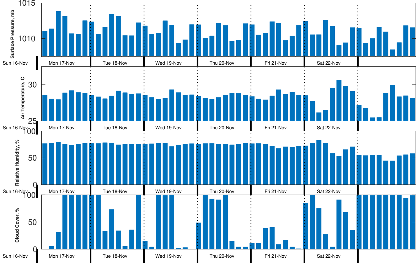
Met Forecast for CSA (ONHYM) PPL EBS - Guinea from 17-Nov-2025 00:00:00 to 24-Nov-2025 00:00:00
