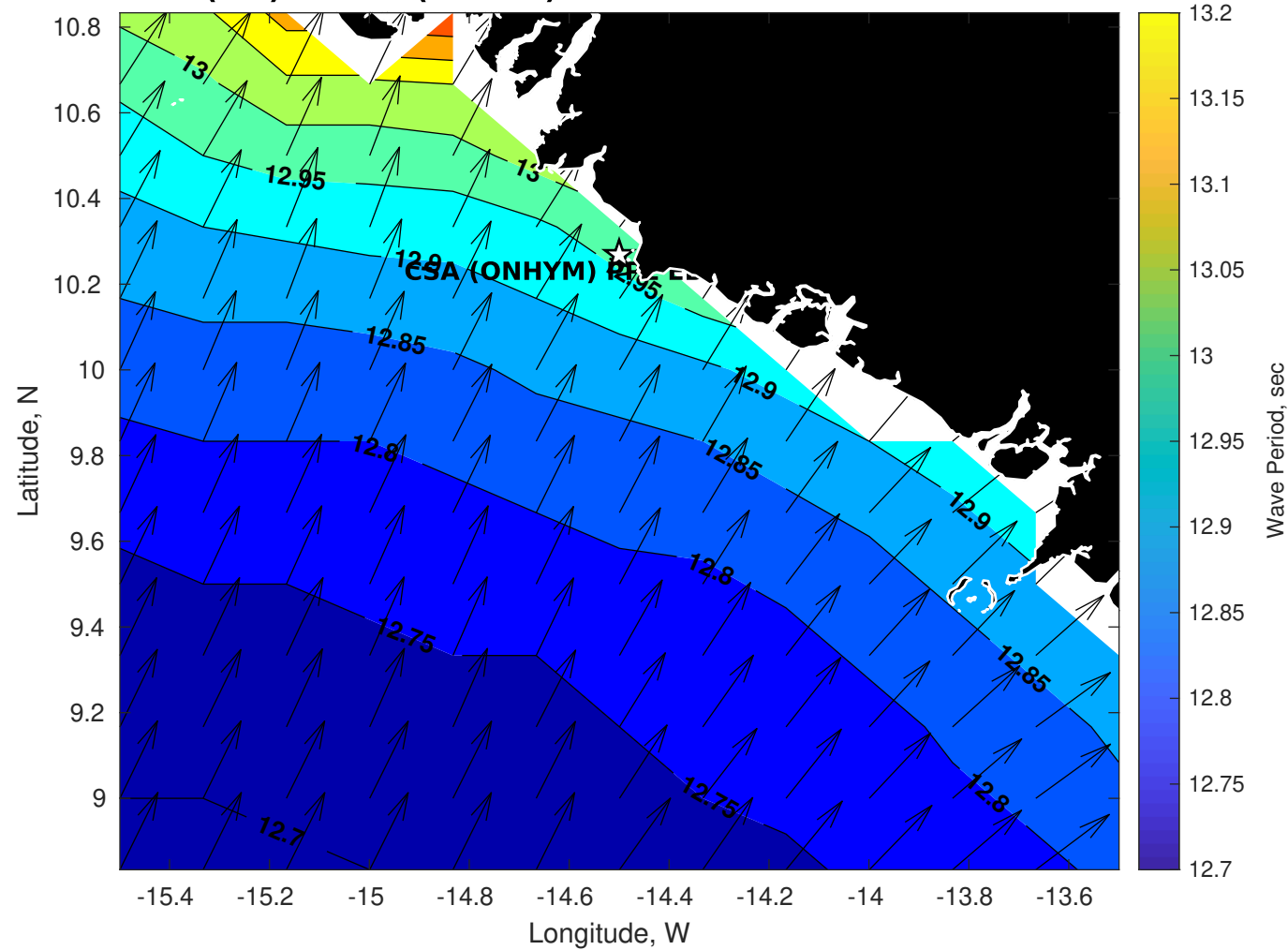
Wave Period (sec) for CSA (ONHYM) PPL EBS - Guinea at 17-Nov-2025 09:00:00
