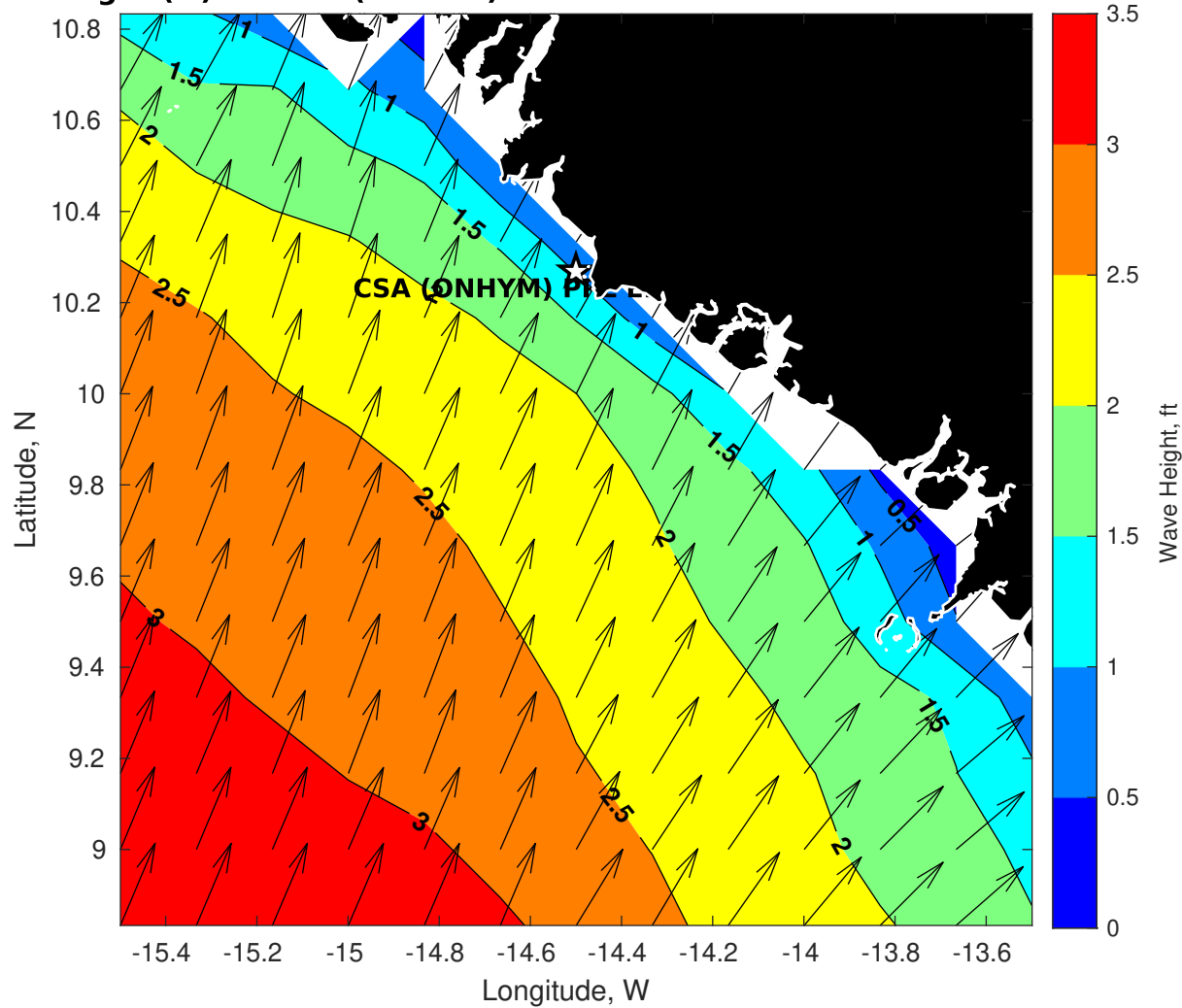
Wave Height (ft) for CSA (ONHYM) PPL EBS - Guinea at 17-Nov-2025 09:00:00
