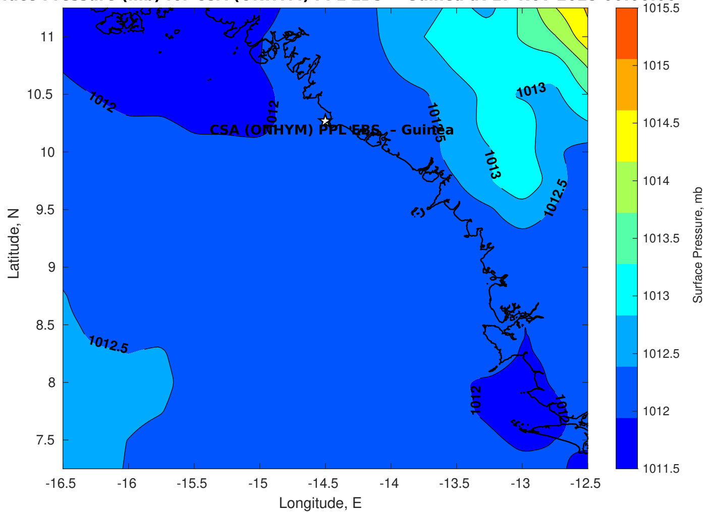
Surface Pressure (mb) for CSA (ONHYM) PPL EBS - Guinea at 17-Nov-2025 00:00:00
