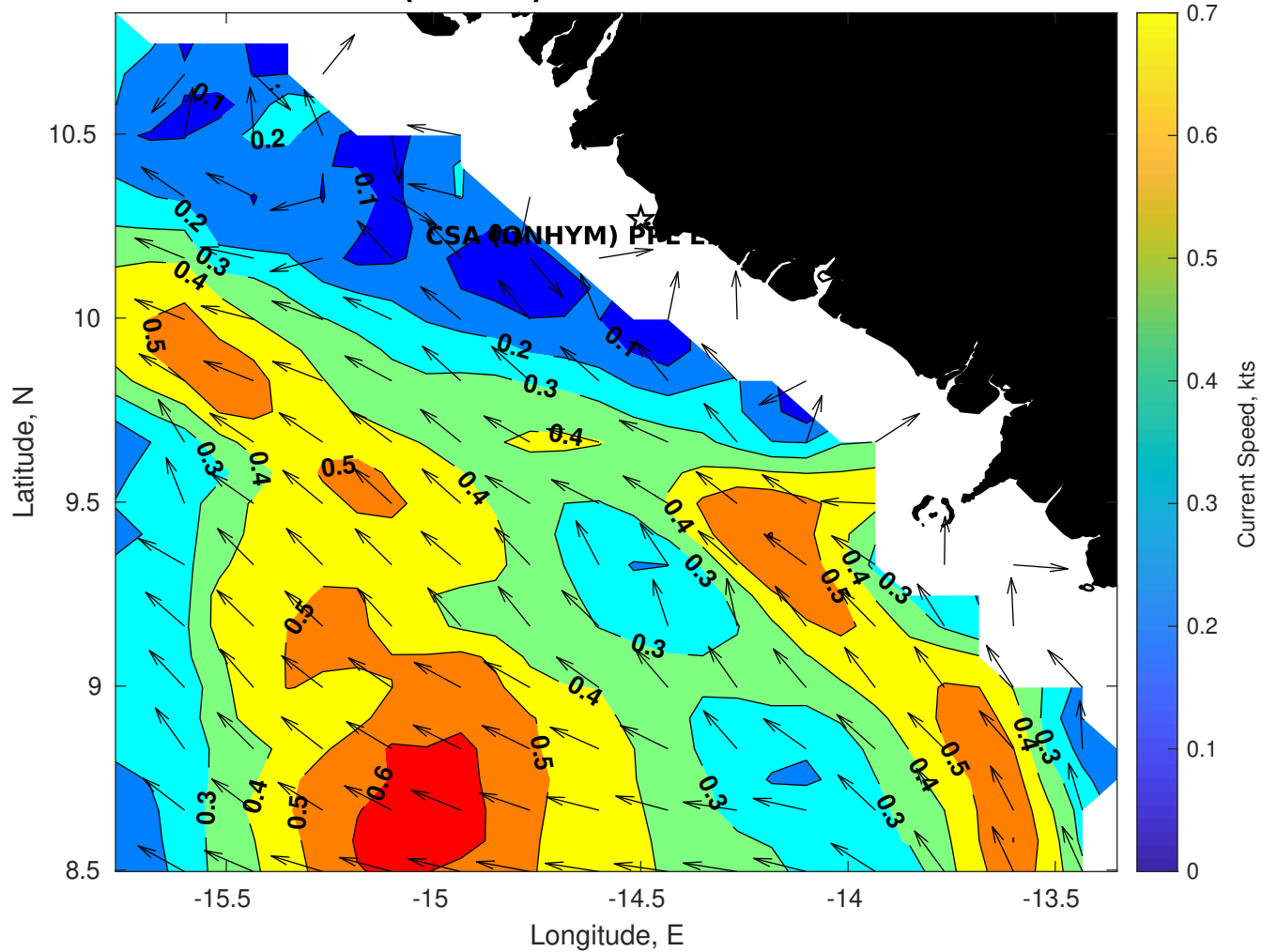
Surface Currents for CSA (ONHYM) PPL EBS - Guinea at 15-Nov-2025 00:00:00
