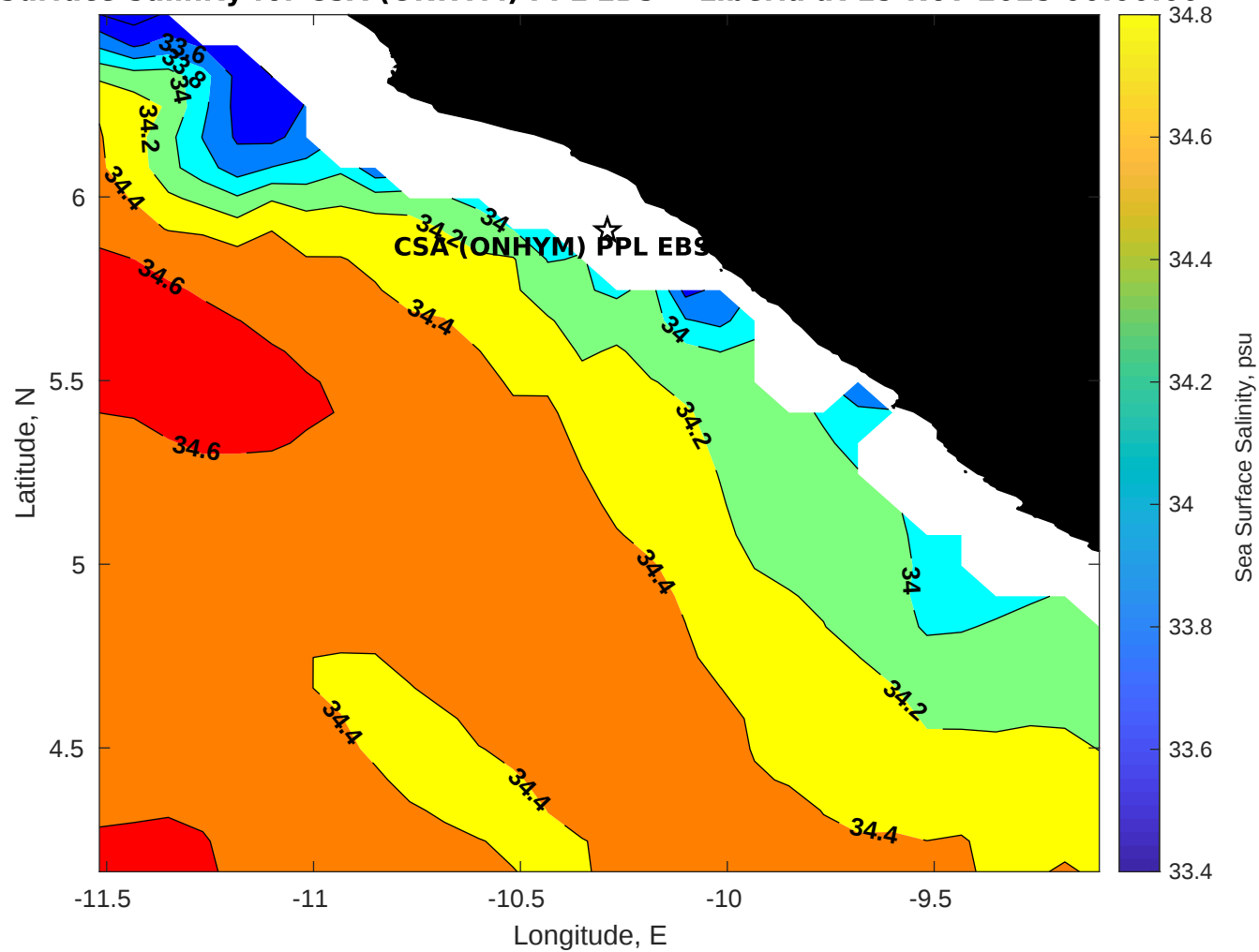
Surface Salinity for CSA (ONHYM) PPL EBS - Liberia at 15-Nov-2025 00:00:00
