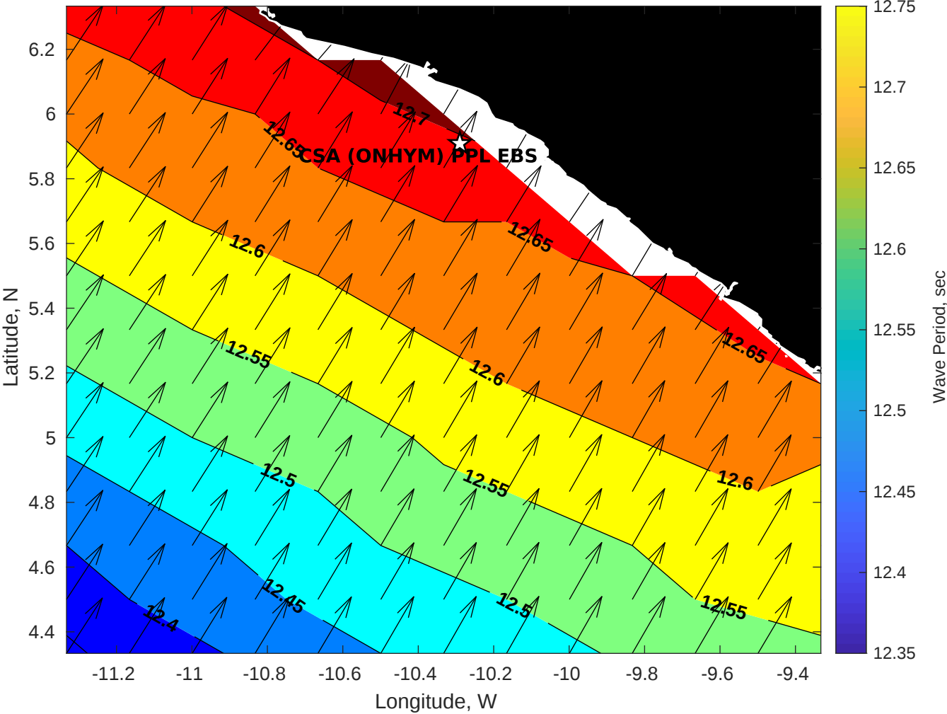
Wave Period (sec) for CSA (ONHYM) PPL EBS - Liberia at 17-Nov-2025 09:00:00
