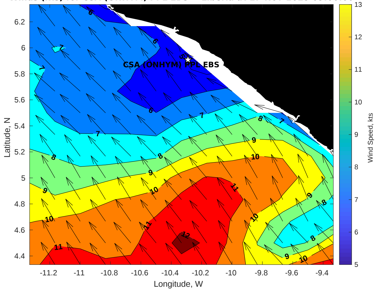
Winds (kts) for CSA (ONHYM) PPL EBS - Liberia at 17-Nov-2025 09:00:00
