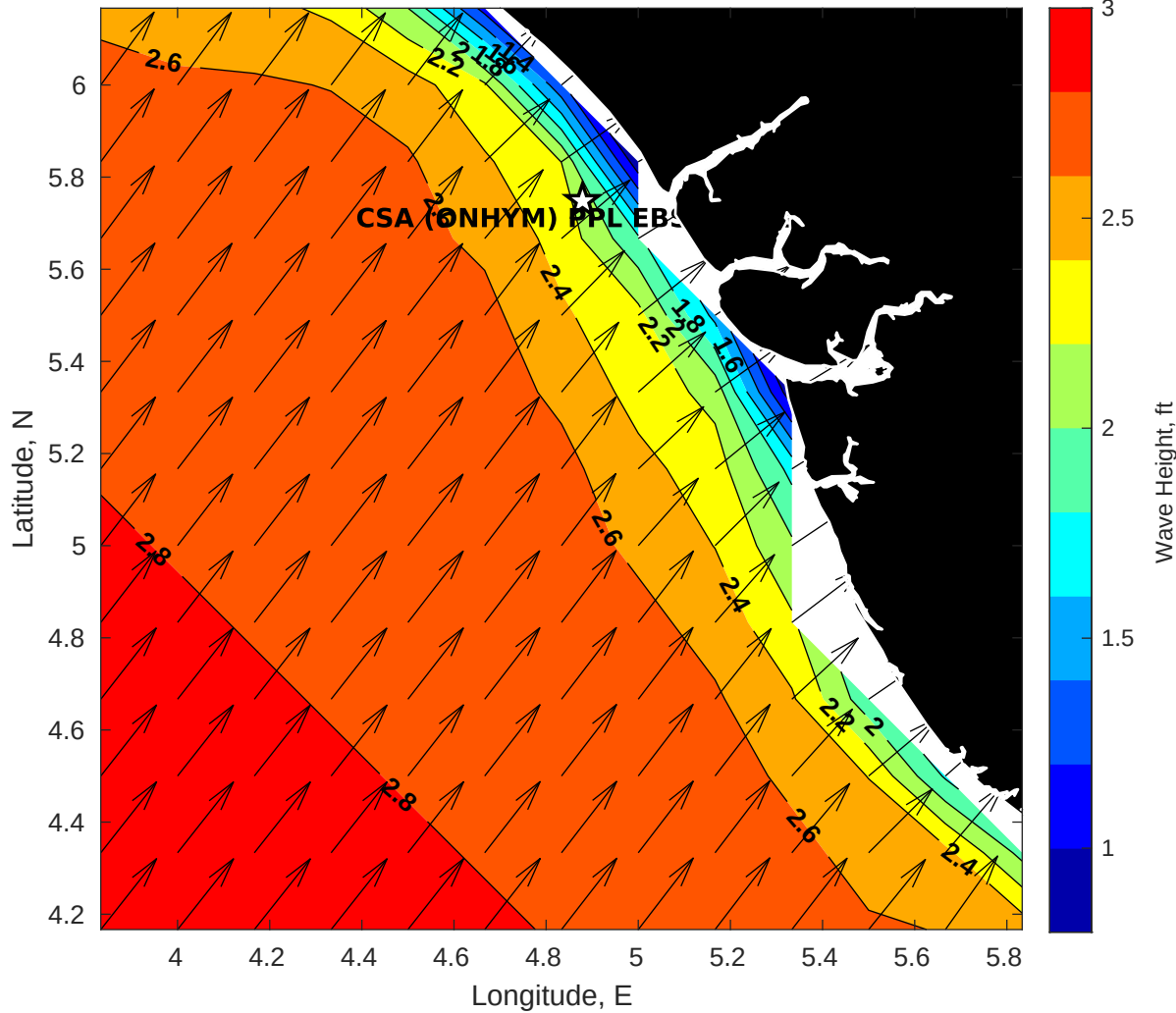
Wave Height (ft) for CSA (ONHYM) PPL EBS - Nigeria at 17-Nov-2025 09:00:00
