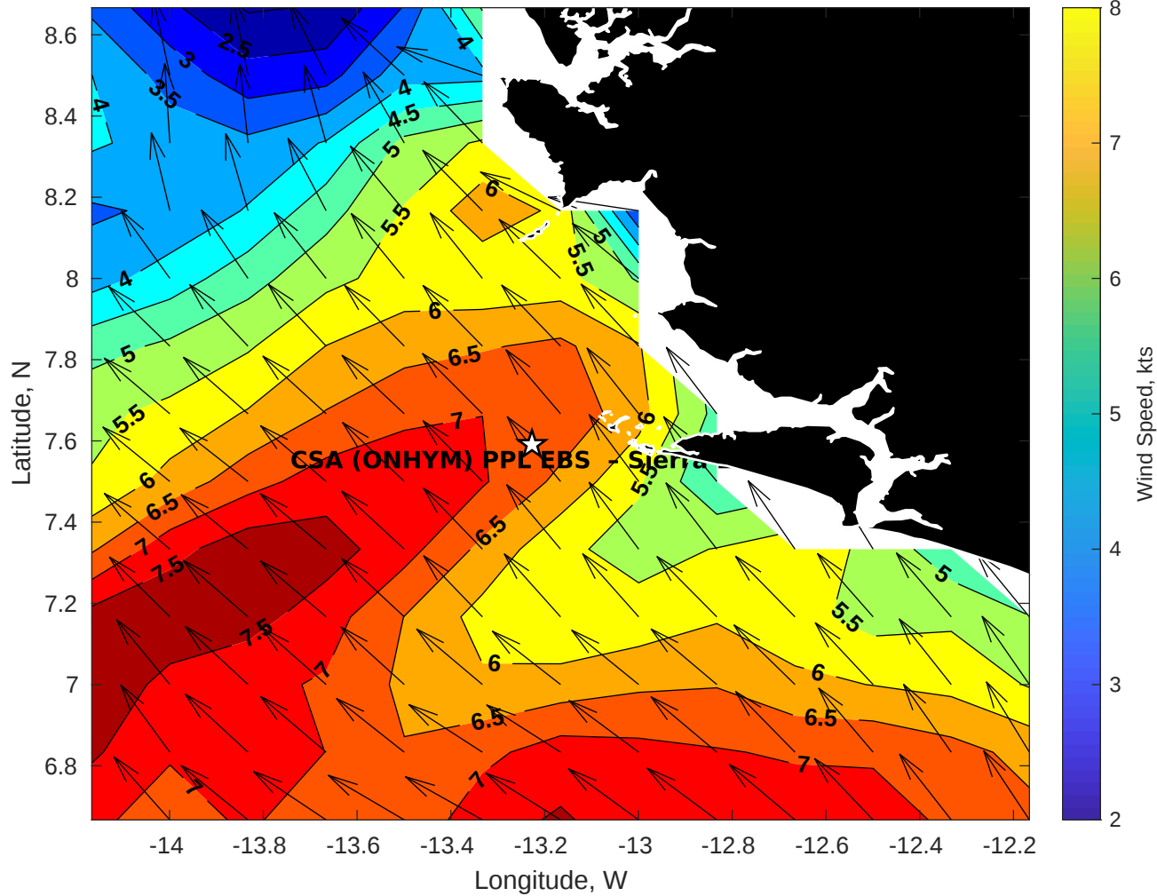
Winds (kts) for CSA (ONHYM) PPL EBS - Sierra Leone at 17-Nov-2025 09:00:00
