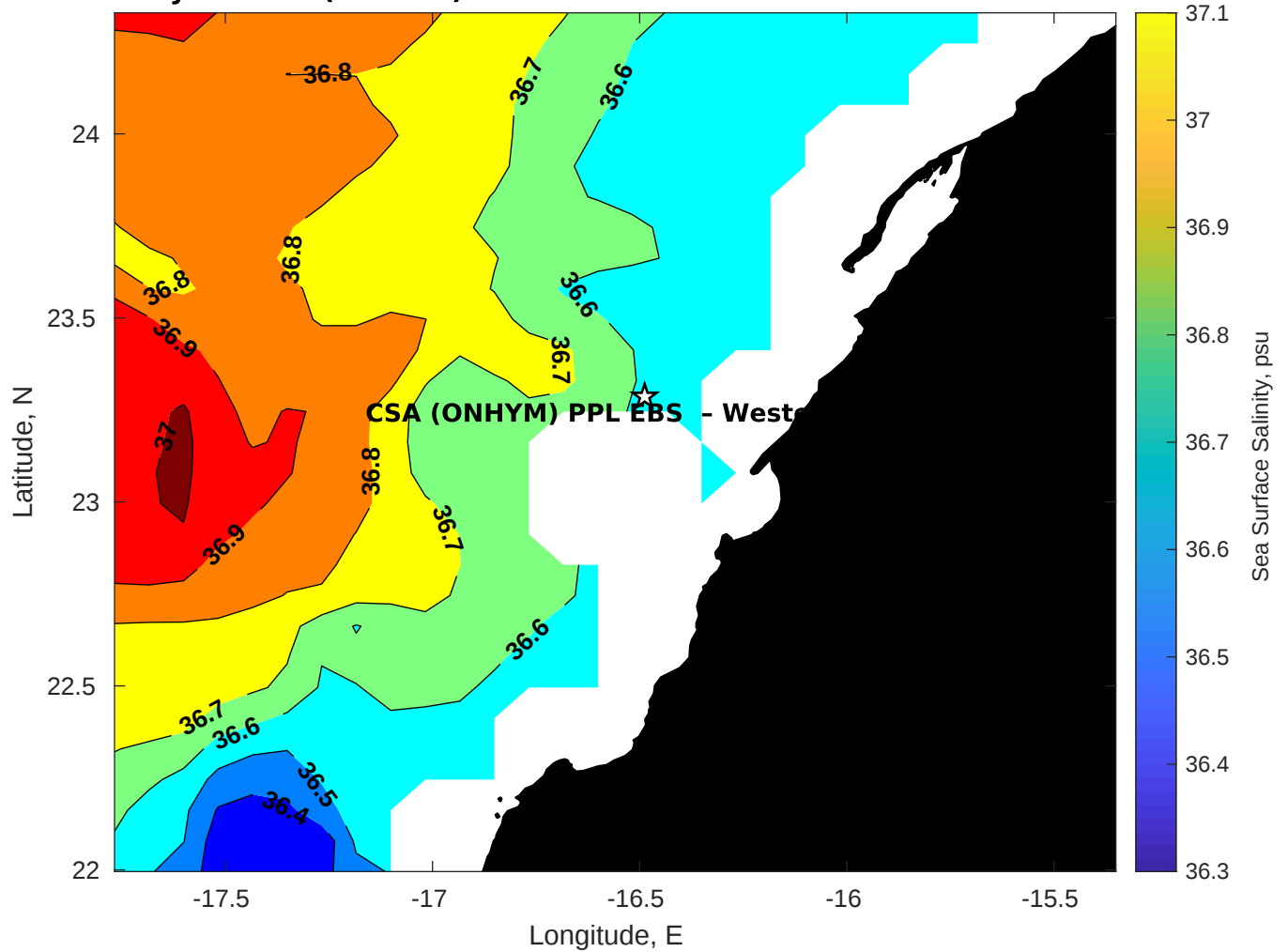
Surface Salinity for CSA (ONHYM) PPL EBS - Western Sahara at 15-Nov-2025 00:00:00
