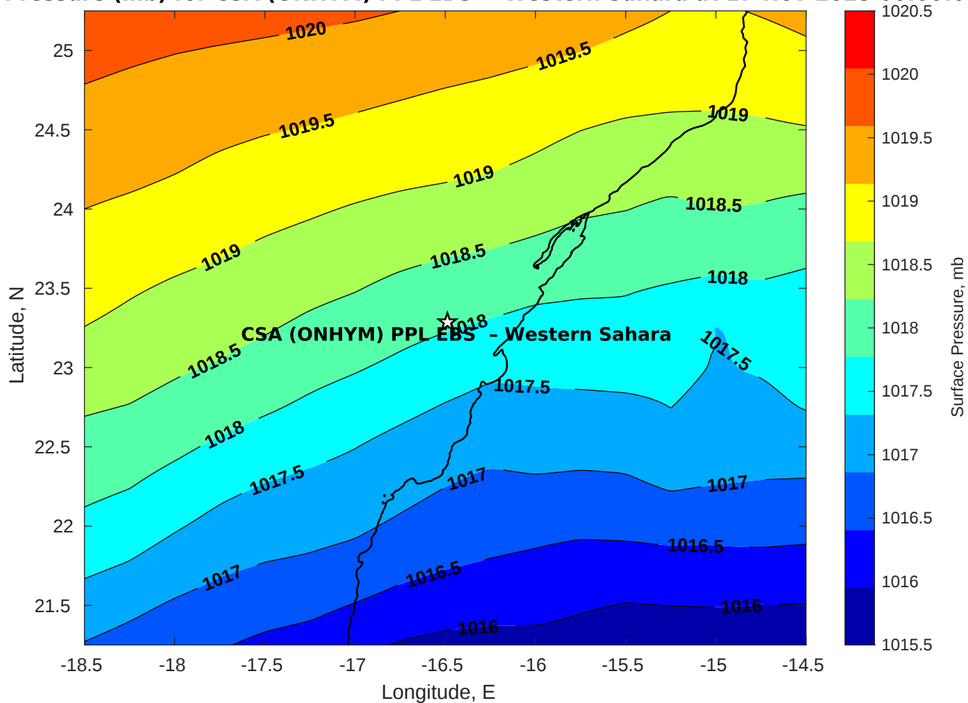
Surface Pressure (mb) for CSA (ONHYM) PPL EBS - Western Sahara at 17-Nov-2025 00:00:00
