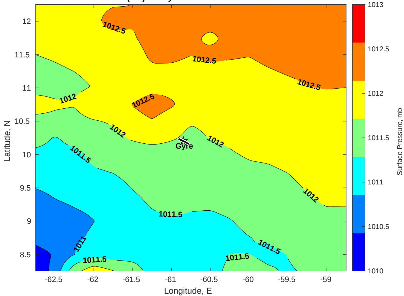
Surface Pressure (mb) for Gyre at 17-Nov-2025 00:00:00
