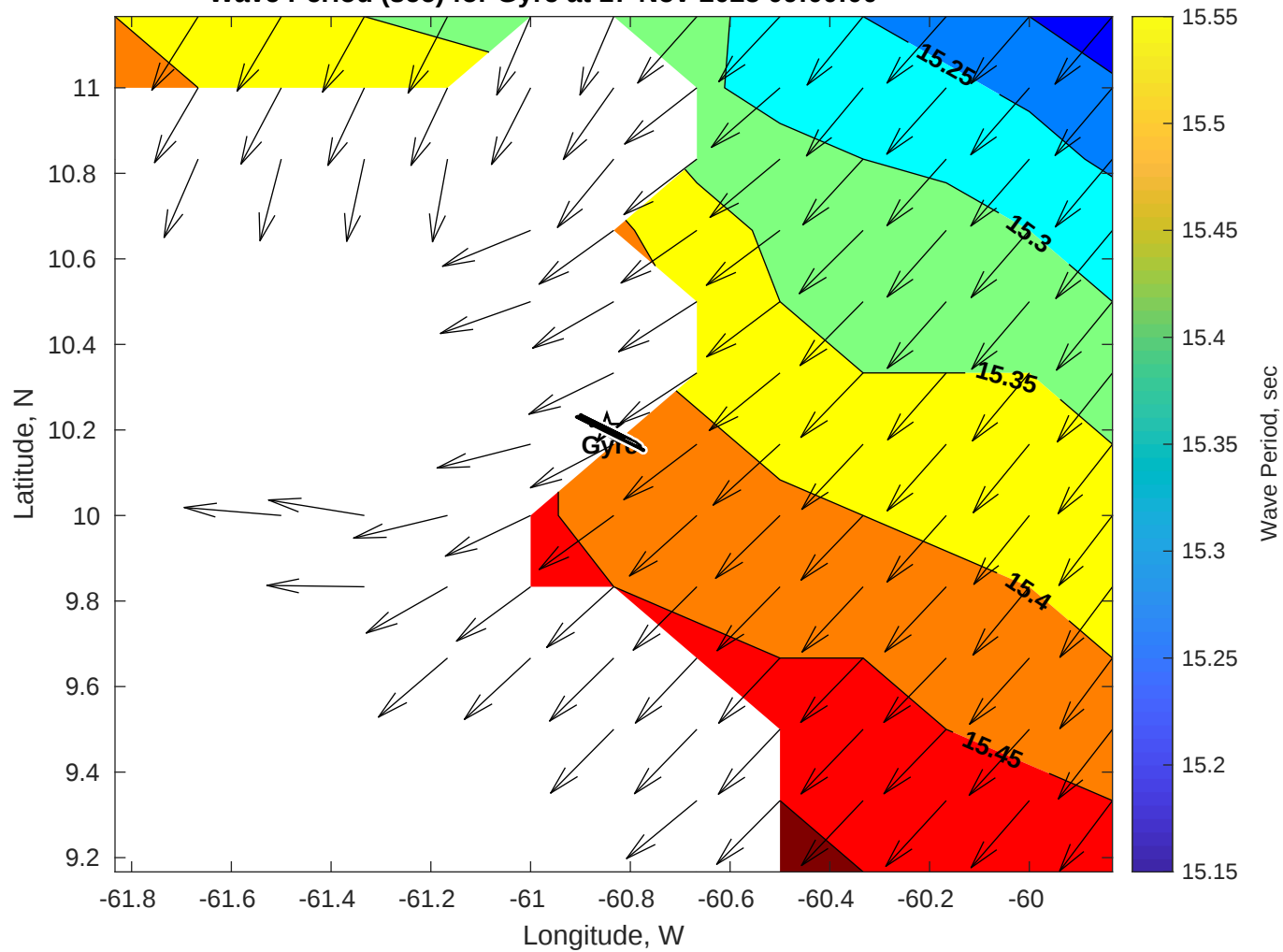
Wave Period (sec) for Gyre at 17-Nov-2025 09:00:00
