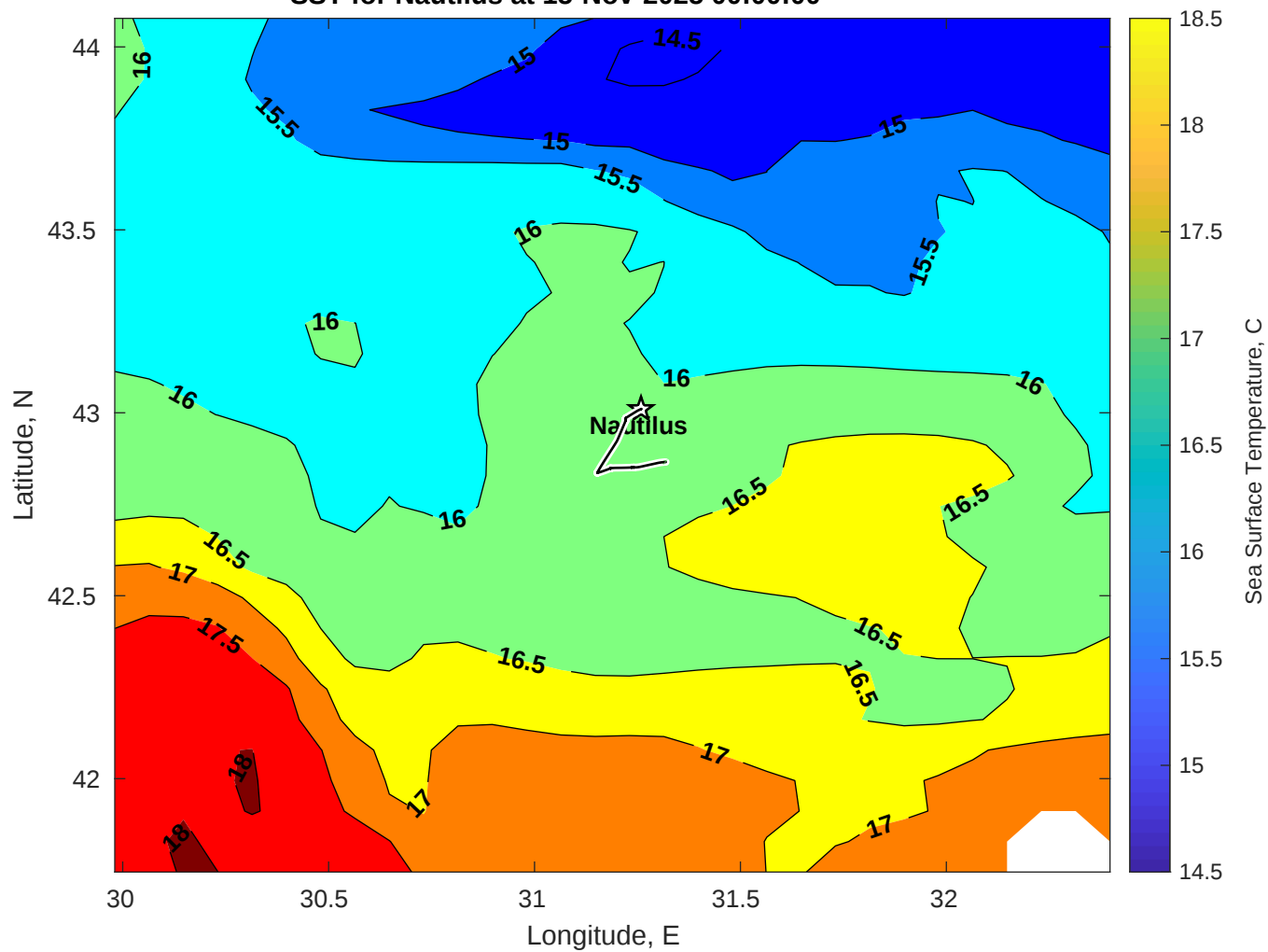
SST for Nautilus at 15-Nov-2025 00:00:00
