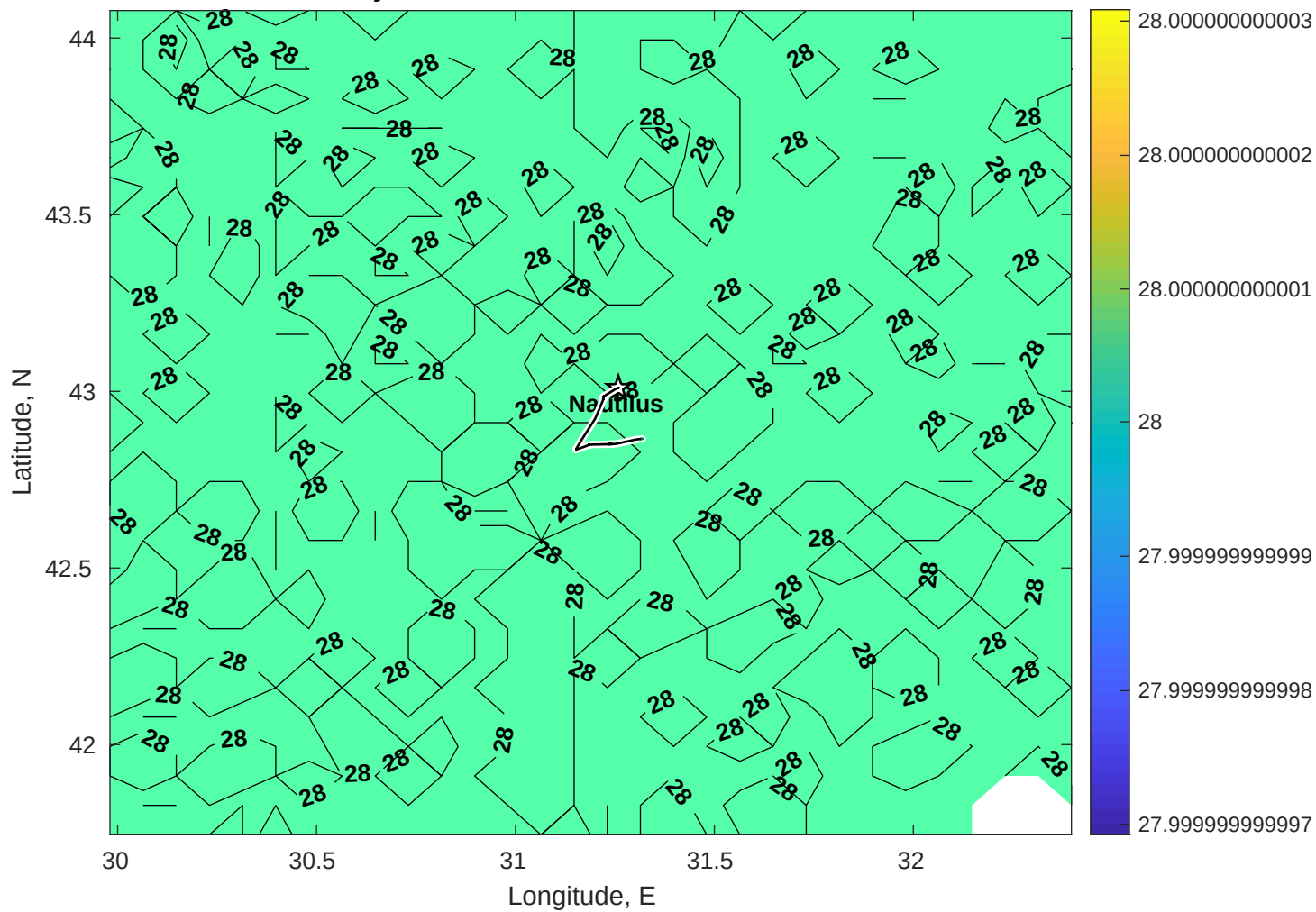
Surface Salinity for Nautilus at 15-Nov-2025 00:00:00
