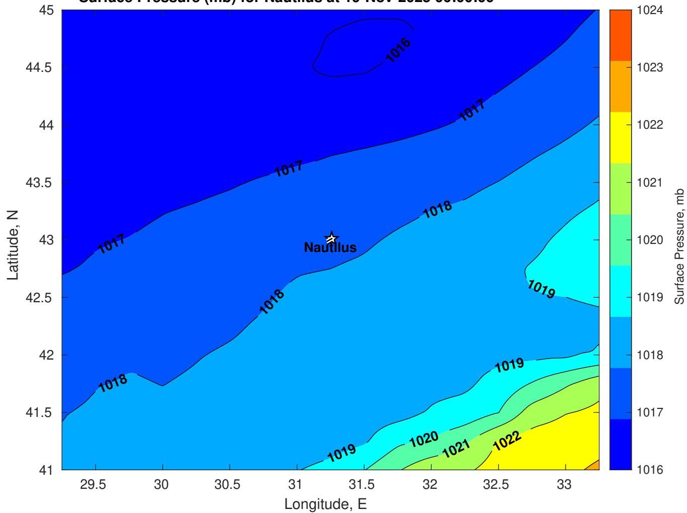
Surface Pressure (mb) for Nautilus at 19-Nov-2025 00:00:00
