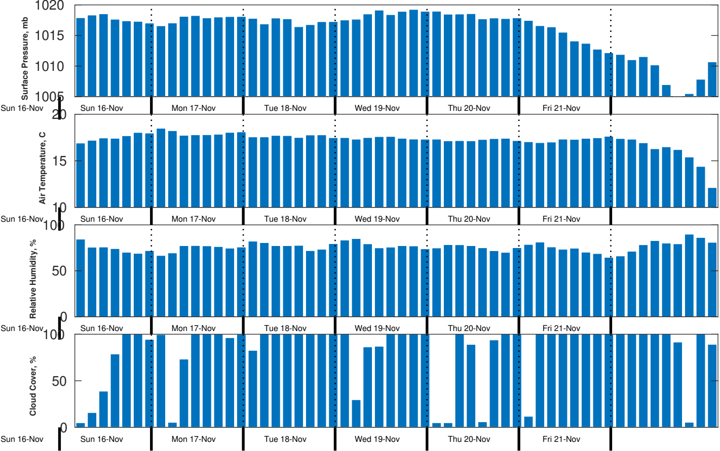
Met Forecast for Nautilus from 17-Nov-2025 00:00:00 to 24-Nov-2025 00:00:00
