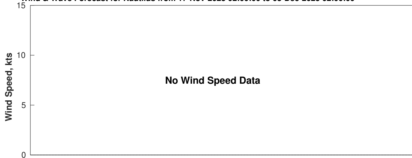
Wind & Wave Forecast for Nautilus from 17-Nov-2025 02:00:00 to 03-Dec-2025 02:00:00
