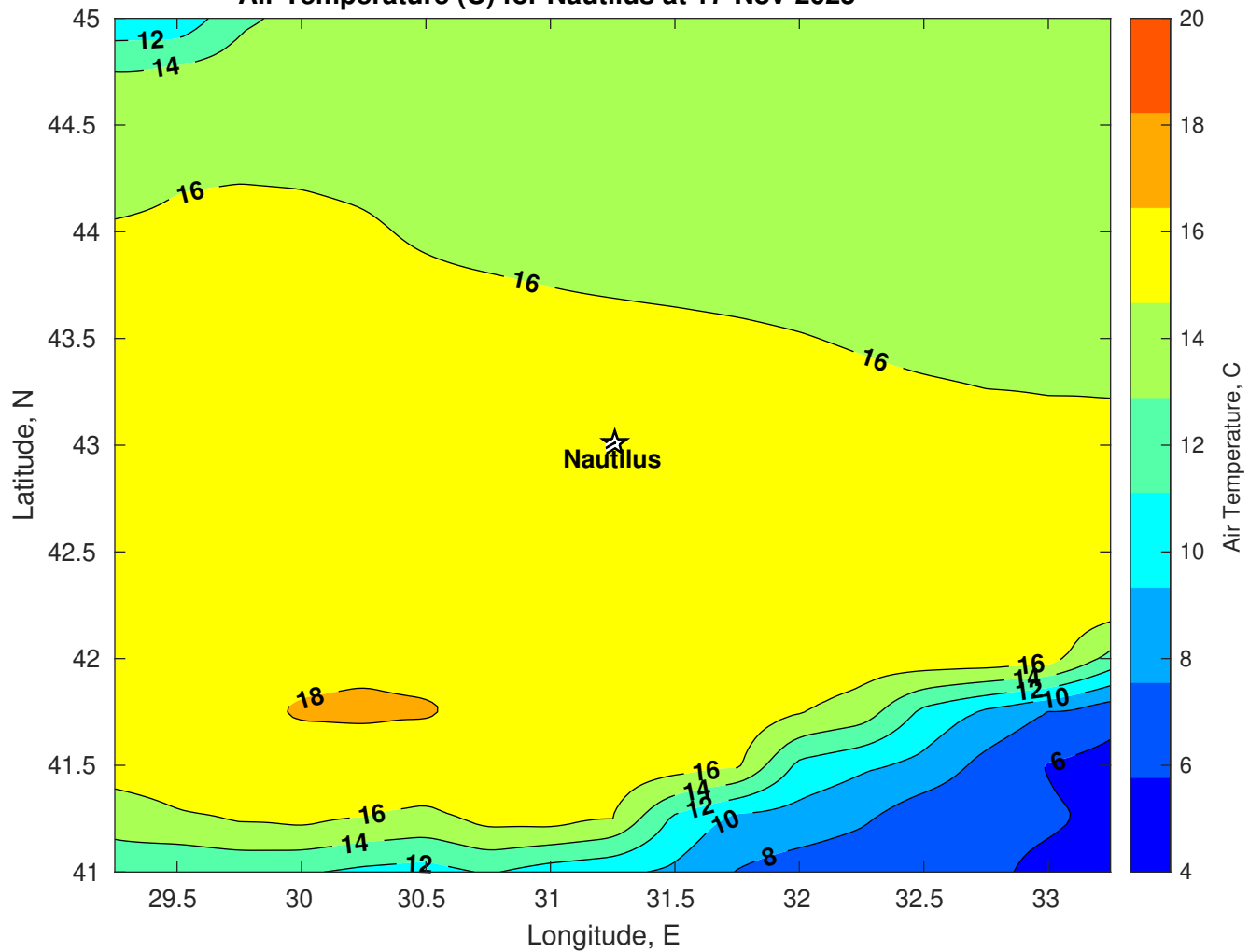
Air Temperature (C) for Nautilus at 17-Nov-2025
