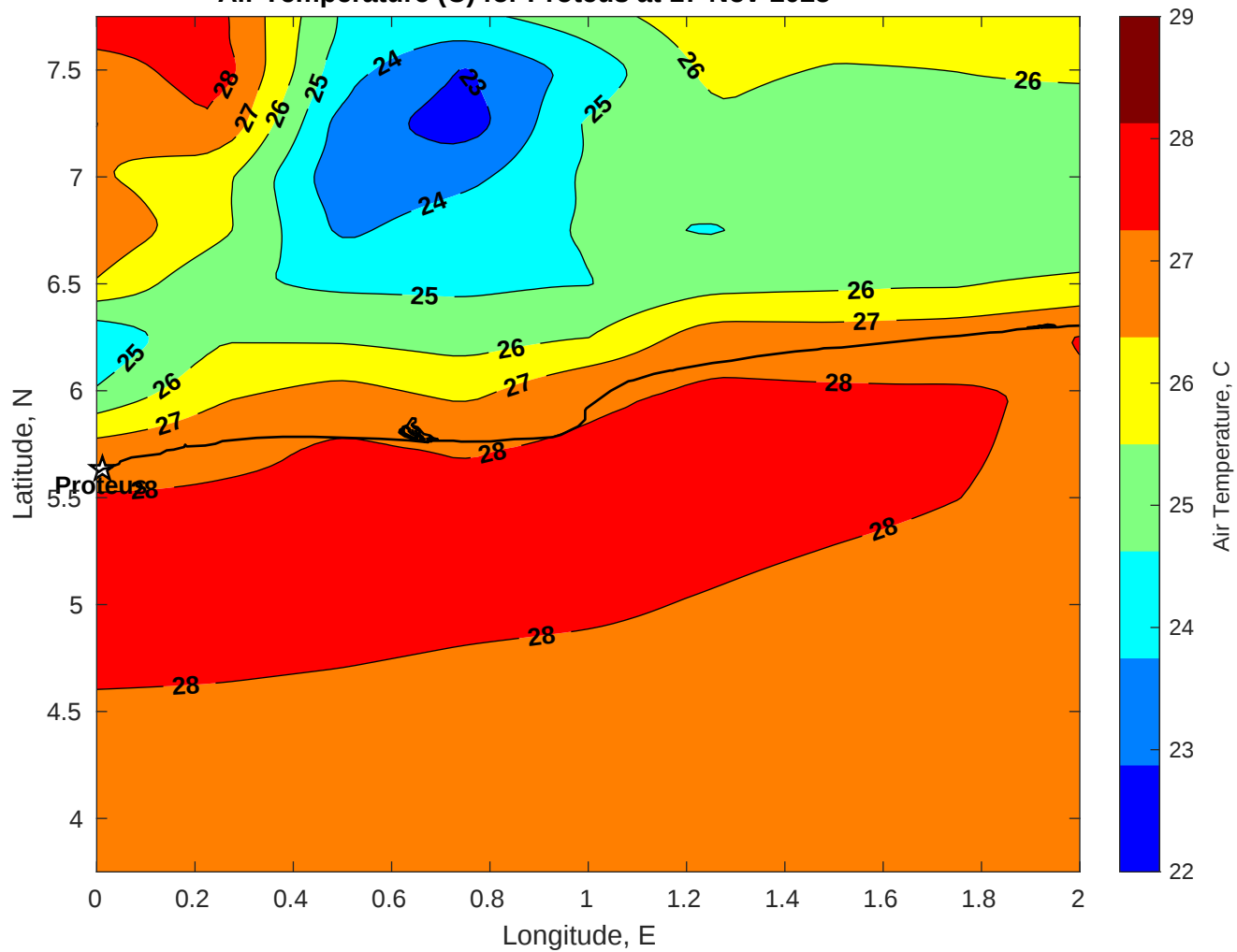
Air Temperature (C) for Proteus at 17-Nov-2025
