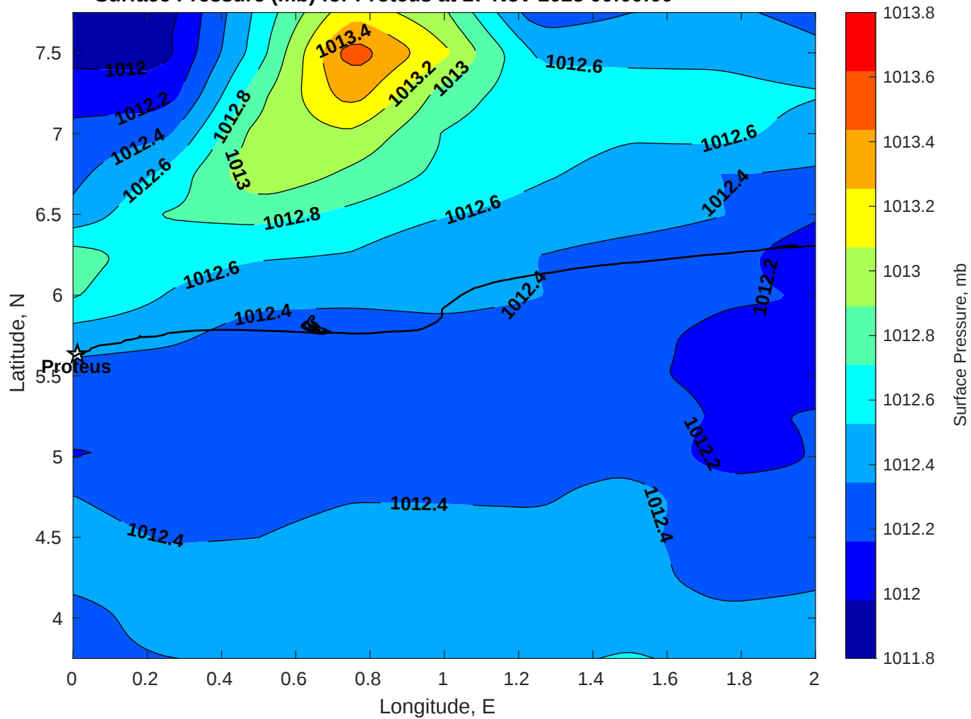
Surface Pressure (mb) for Proteus at 17-Nov-2025 00:00:00
