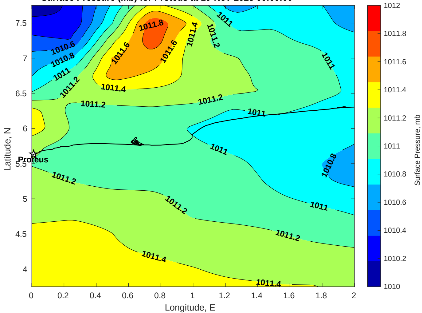
Surface Pressure (mb) for Proteus at 19-Nov-2025 00:00:00
