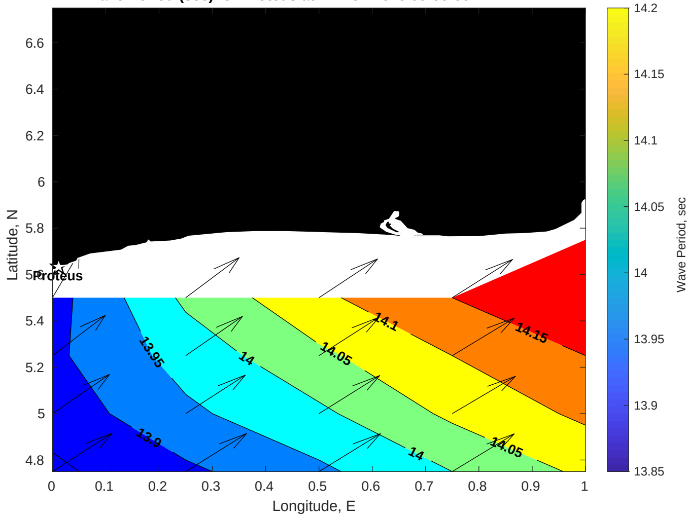
Wave Period (sec) for Proteus at 17-Nov-2025 09:00:00
