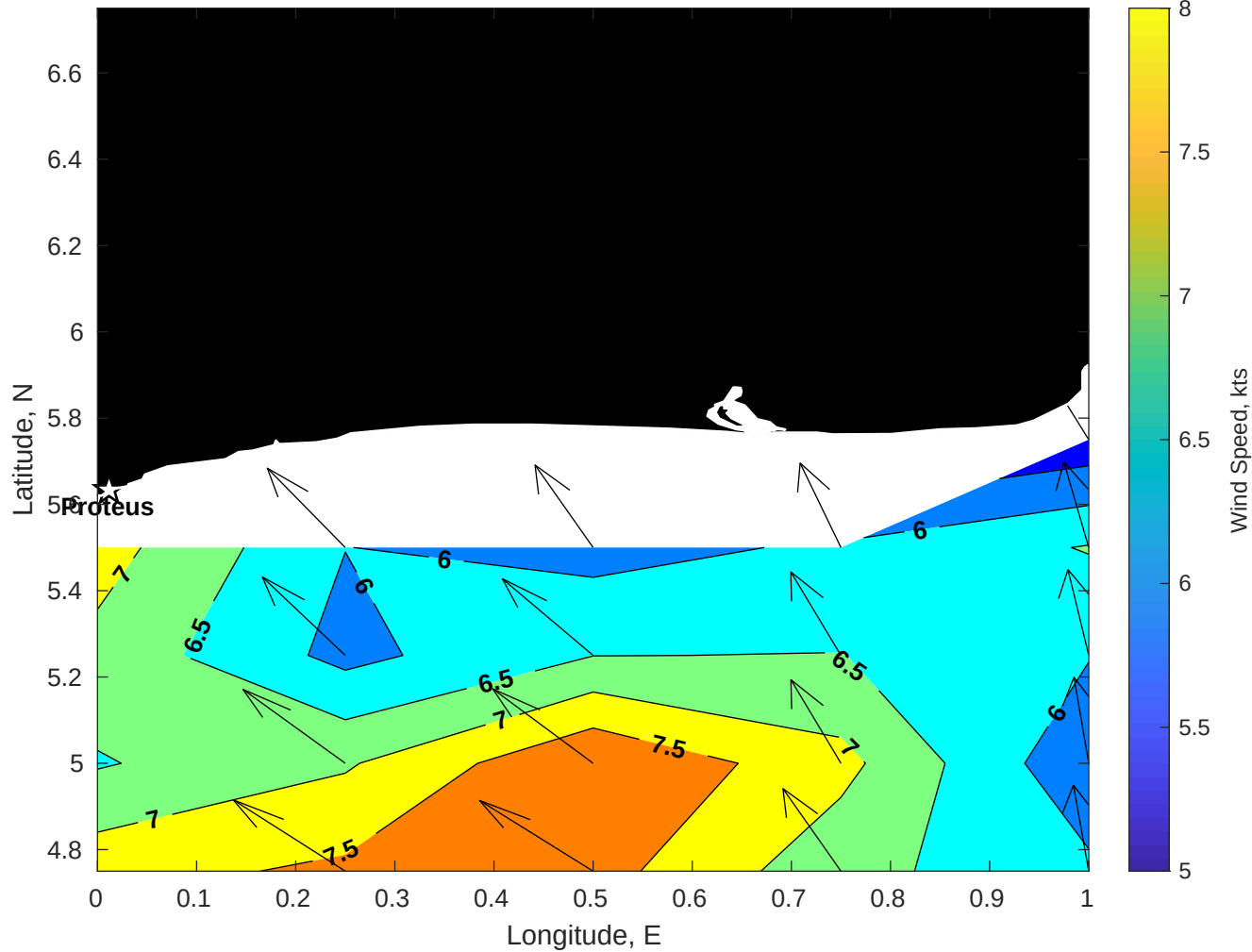
Winds (kts) for Proteus at 17-Nov-2025 09:00:00
