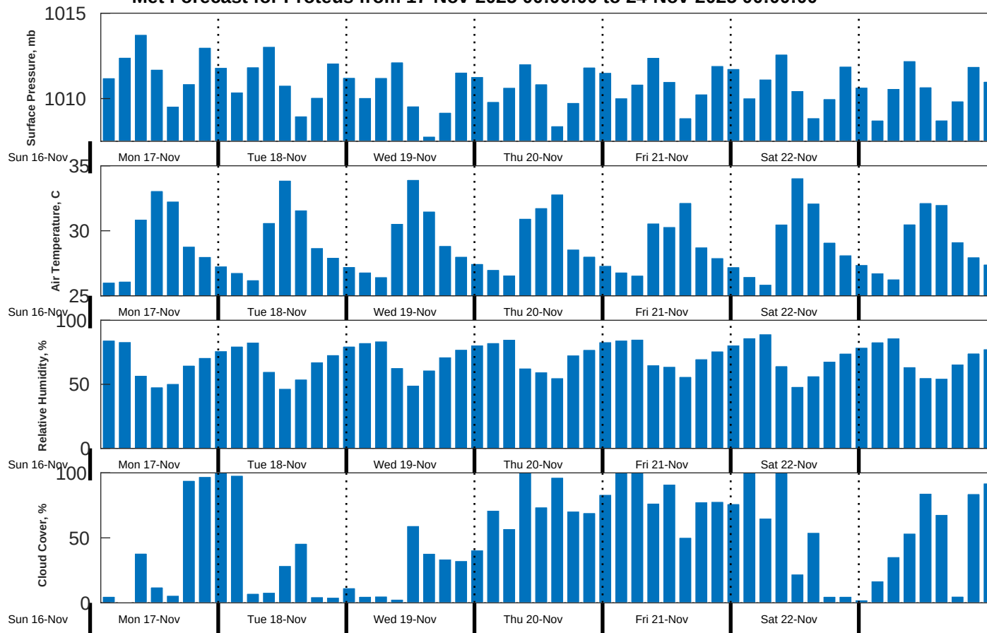
Met Forecast for Proteus from 17-Nov-2025 00:00:00 to 24-Nov-2025 00:00:00
