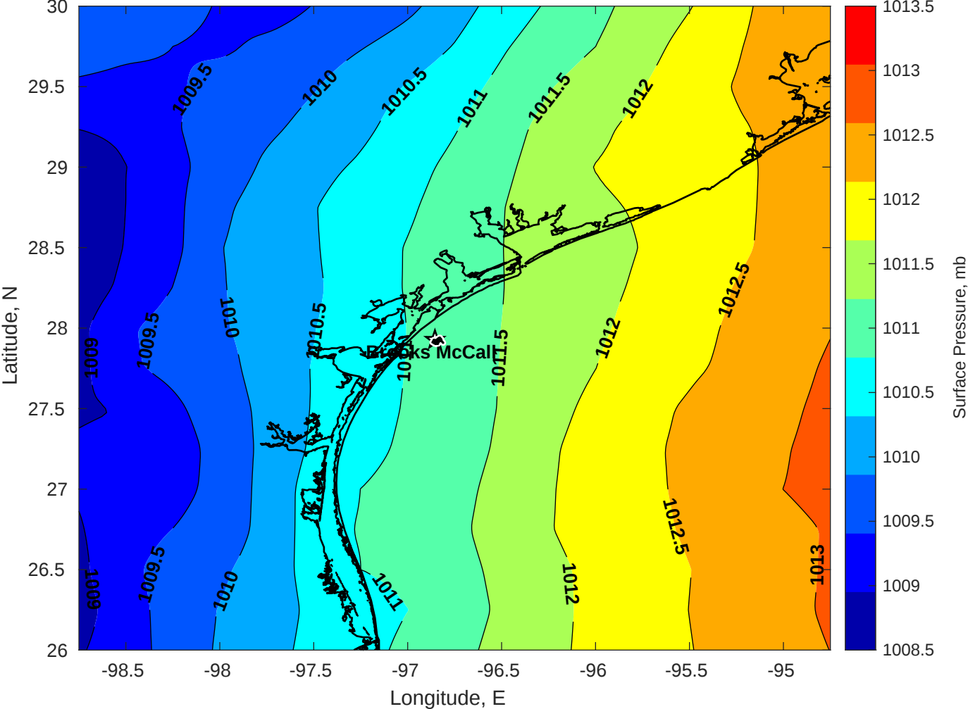
Surface Pressure (mb) for Brooks McCall at 18-Nov-2025 00:00:00
