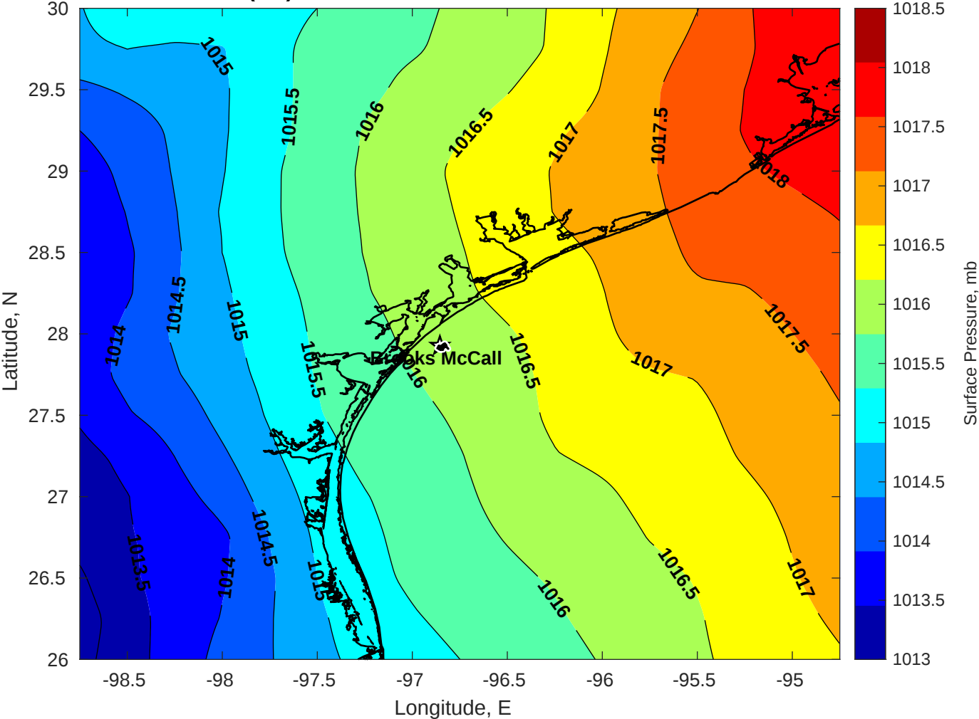
Surface Pressure (mb) for Brooks McCall at 20-Nov-2025 00:00:00
