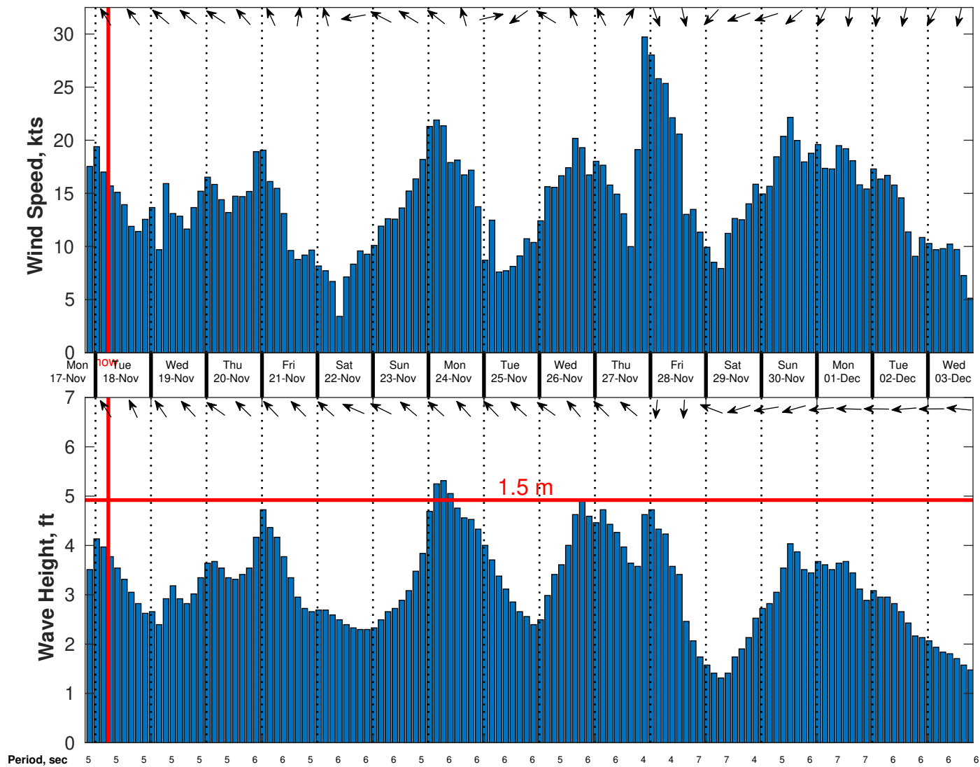
Wind & Wave Forecast for Brooks McCall from 17-Nov-2025 20:00:00 to 03-Dec-2025 20:00:00
