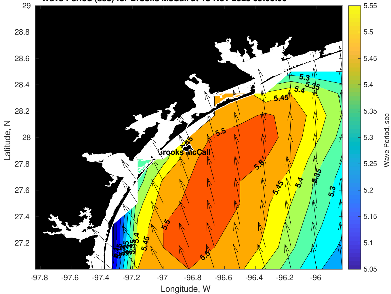
Wave Period (sec) for Brooks McCall at 18-Nov-2025 09:00:00
