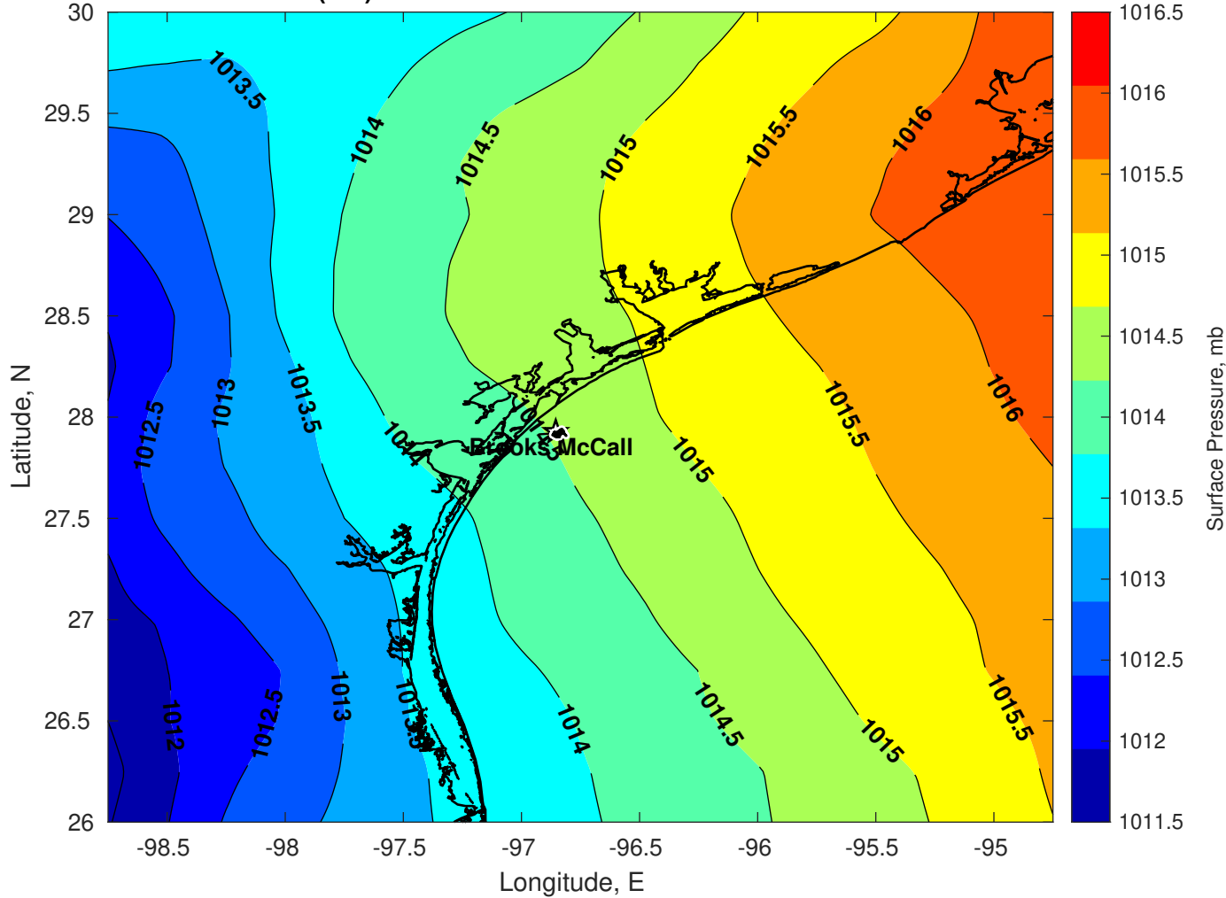
Surface Pressure (mb) for Brooks McCall at 19-Nov-2025 00:00:00
