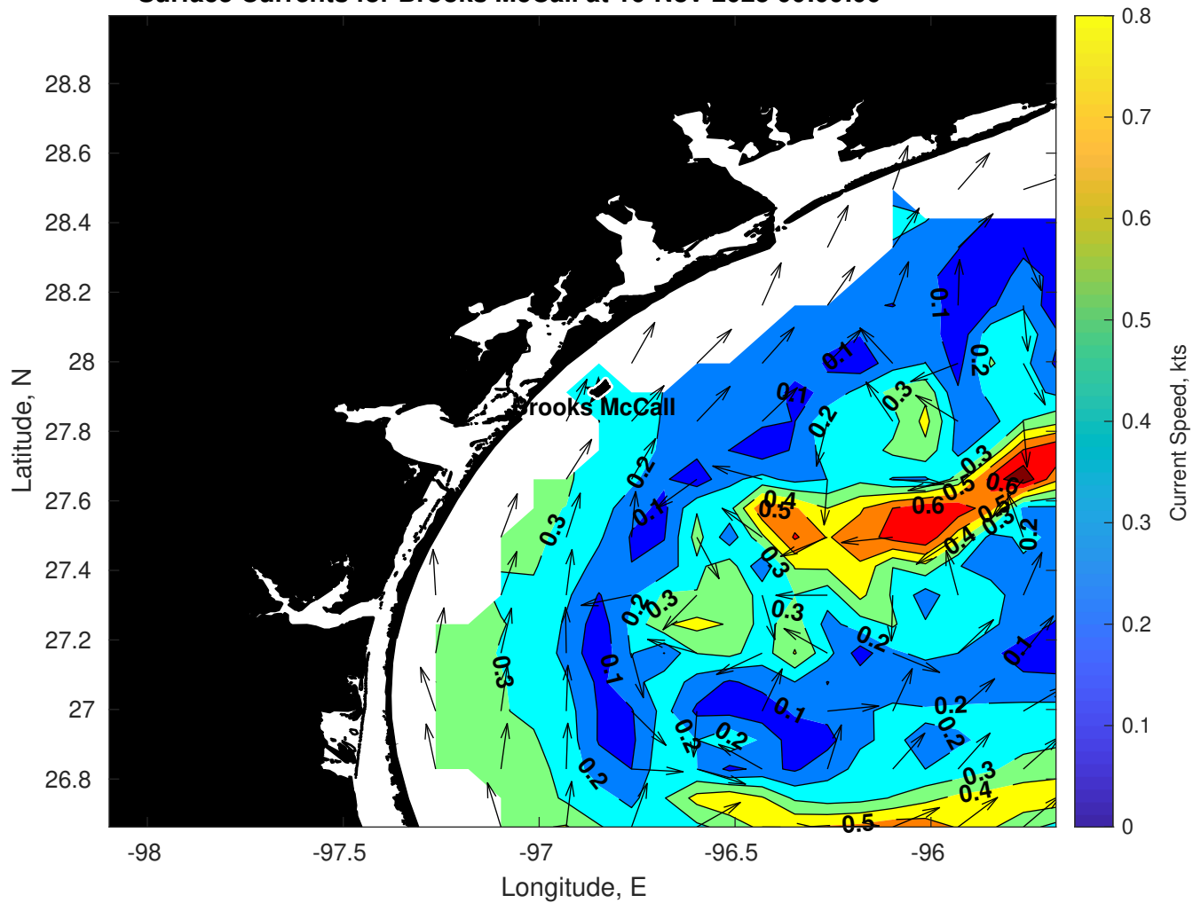
Surface Currents for Brooks McCall at 16-Nov-2025 00:00:00
