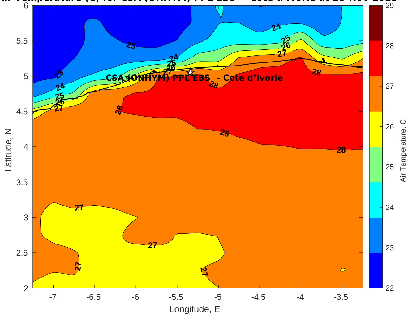
Air Temperature (C) for CSA (ONHYM) PPL EBS - Cote d'Ivoire at 18-Nov-2025
