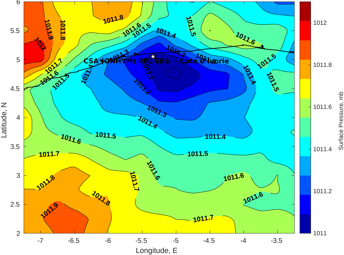
Surface Pressure (mb) for CSA (ONHYM) PPL EBS - Cote d'Ivoire at 20-Nov-2025 00:00:00
