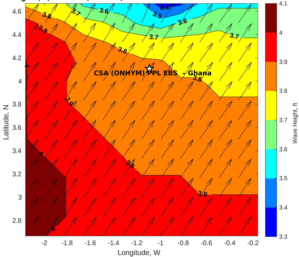
Wave Height (ft) for CSA (ONHYM) PPL EBS - Ghana at 18-Nov-2025 09:00:00
