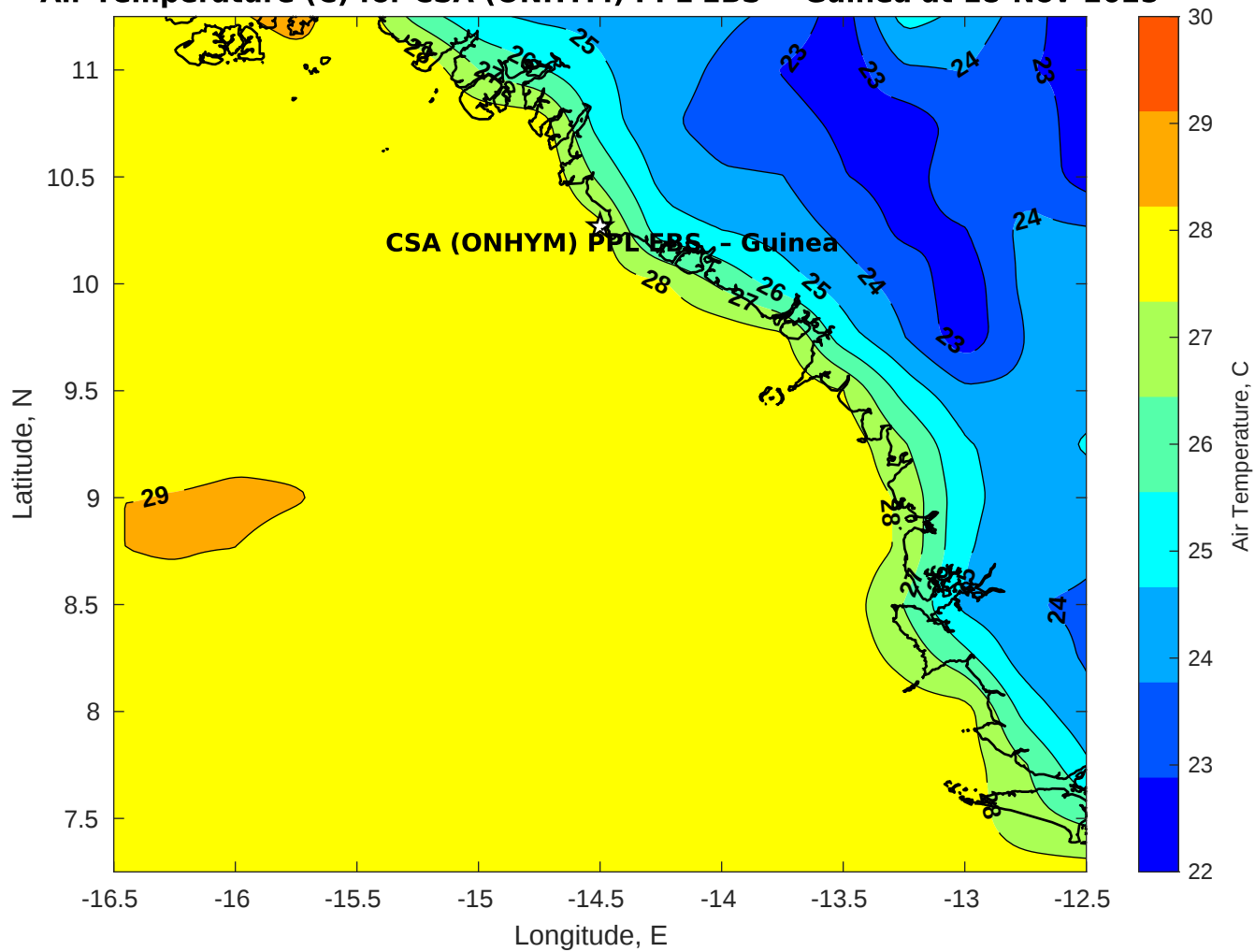
Air Temperature (C) for CSA (ONHYM) PPL EBS - Guinea at 18-Nov-2025
