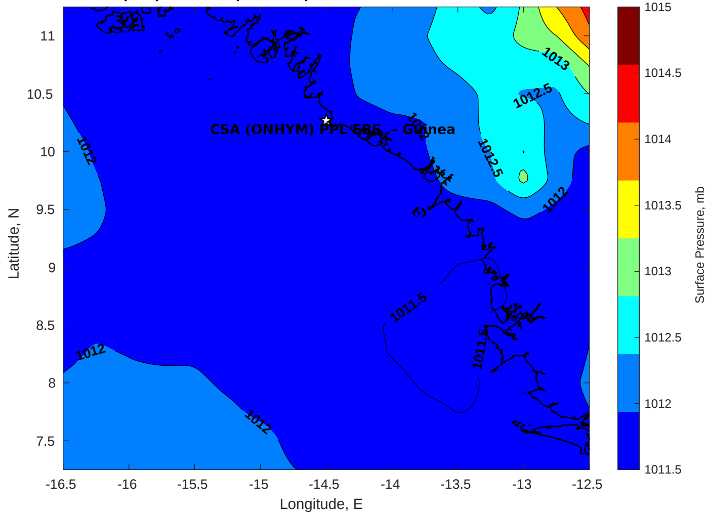
Surface Pressure (mb) for CSA (ONHYM) PPL EBS - Guinea at 18-Nov-2025 00:00:00
