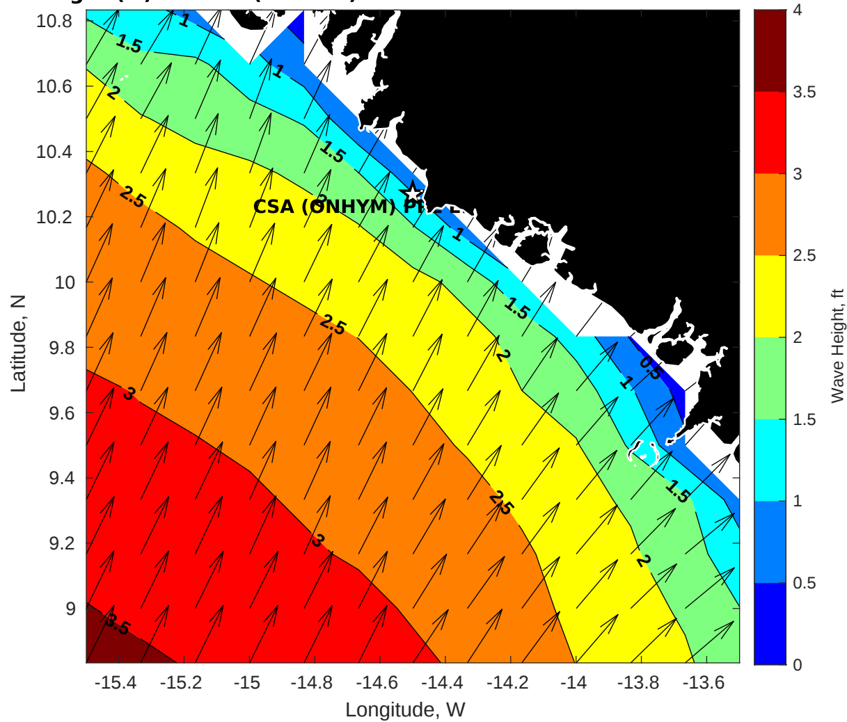
Wave Height (ft) for CSA (ONHYM) PPL EBS - Guinea at 18-Nov-2025 09:00:00
