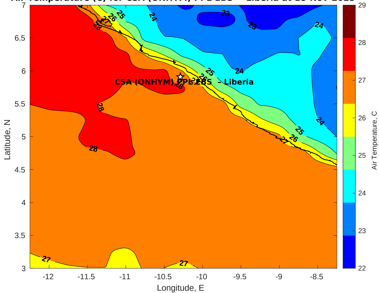
Air Temperature (C) for CSA (ONHYM) PPL EBS - Liberia at 18-Nov-2025
