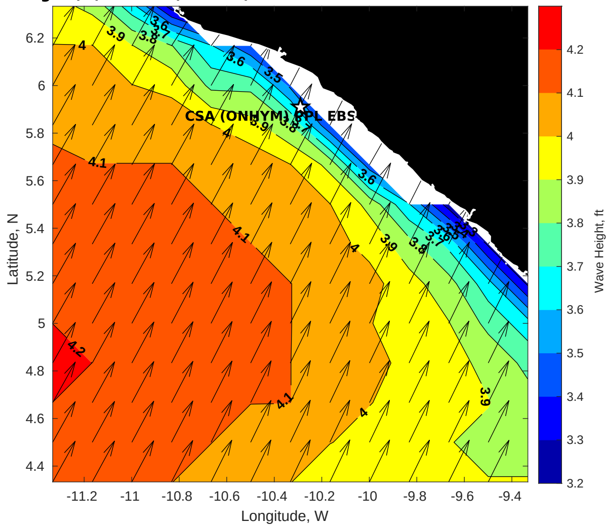
Wave Height (ft) for CSA (ONHYM) PPL EBS - Liberia at 18-Nov-2025 09:00:00
