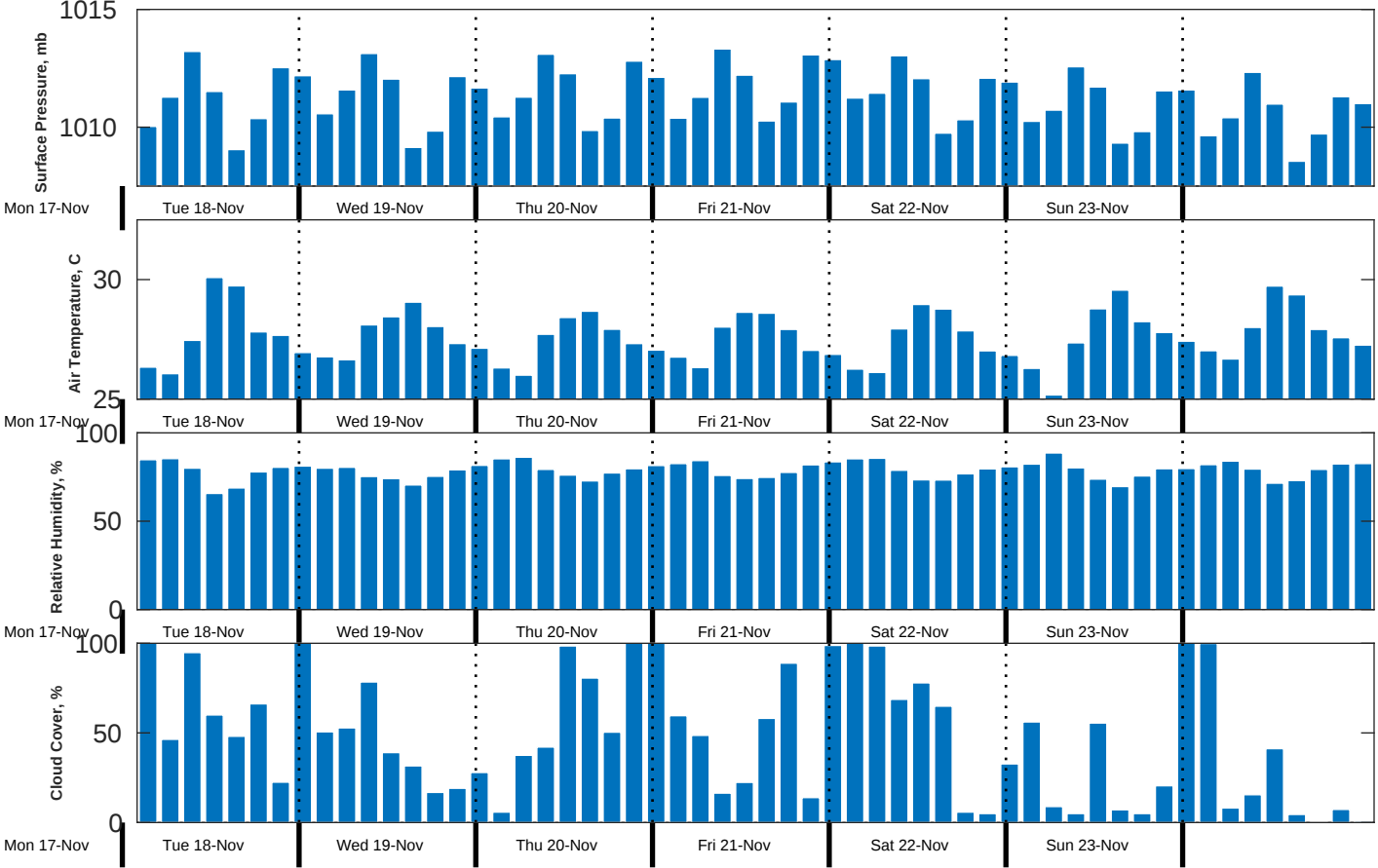
Met Forecast for CSA (ONHYM) PPL EBS - Liberia from 18-Nov-2025 00:00:00 to 25-Nov-2025 00:00:00
