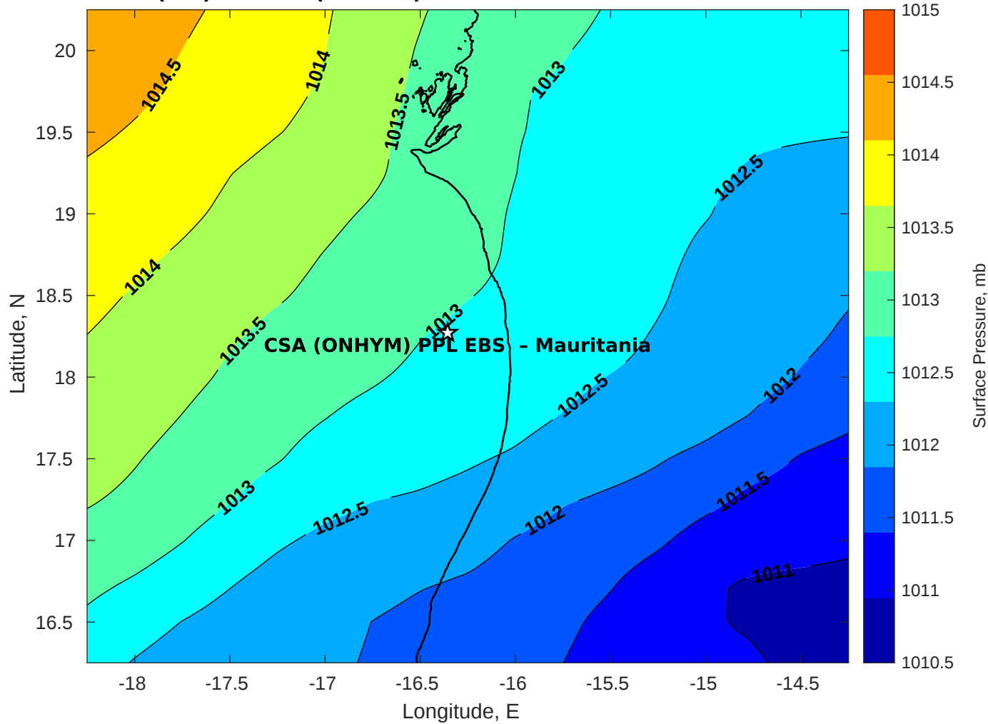
Surface Pressure (mb) for CSA (ONHYM) PPL EBS - Mauritania at 20-Nov-2025 00:00:00
