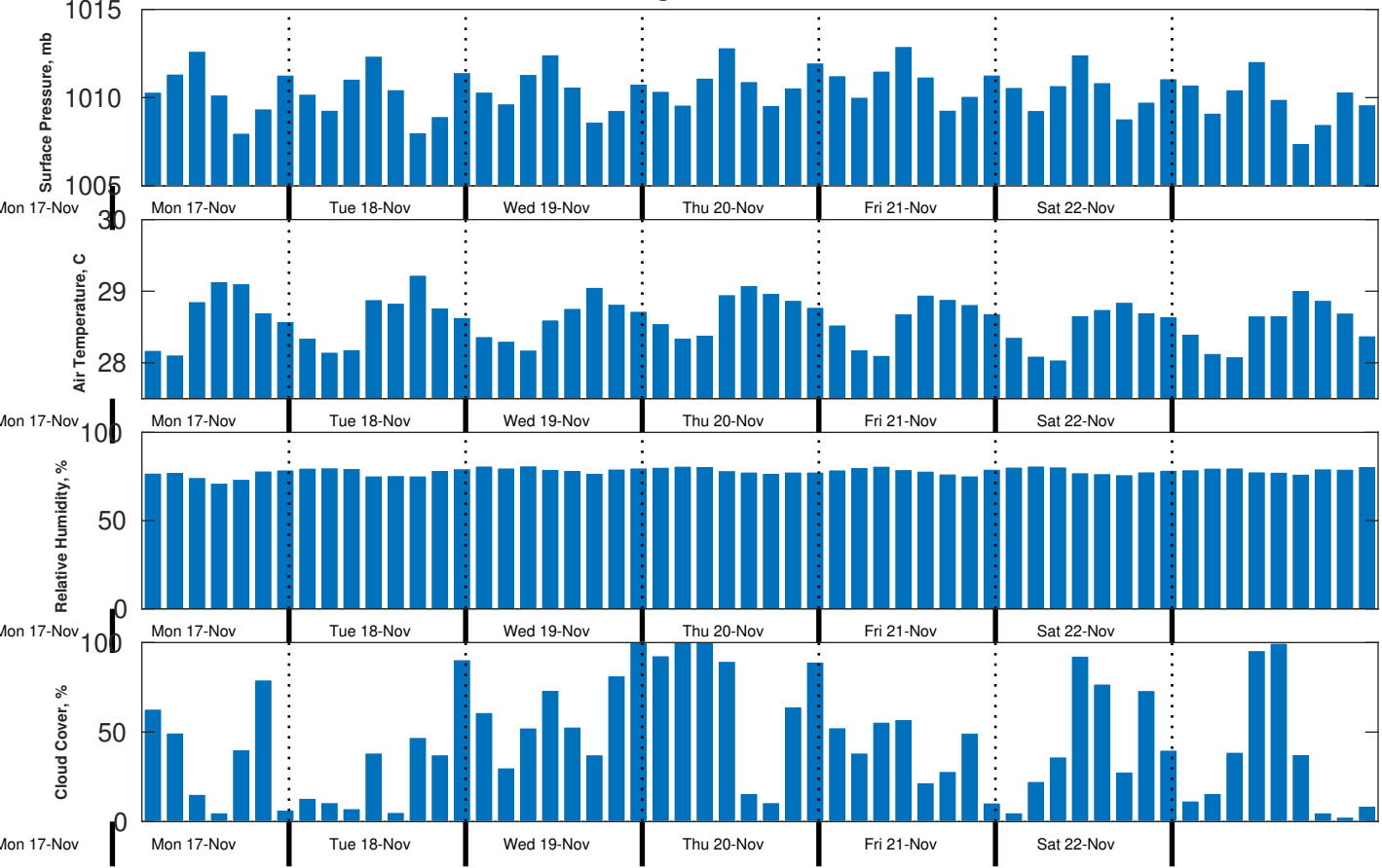
Met Forecast for CSA (ONHYM) PPL EBS - Nigeria from 18-Nov-2025 00:00:00 to 25-Nov-2025 00:00:00
