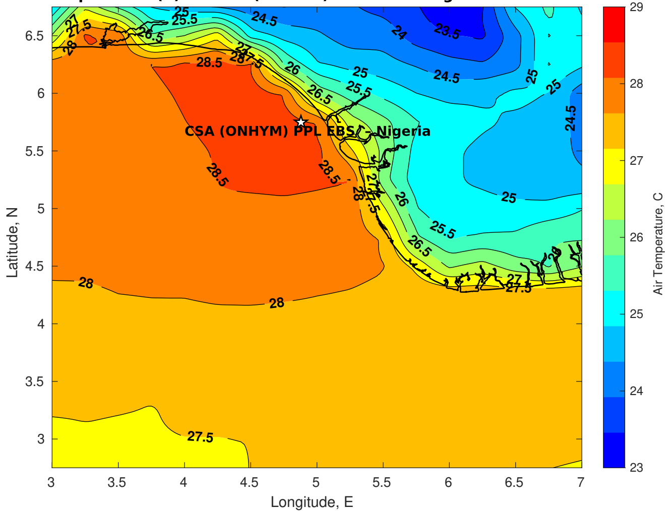
Air Temperature (C) for CSA (ONHYM) PPL EBS - Nigeria at 18-Nov-2025
