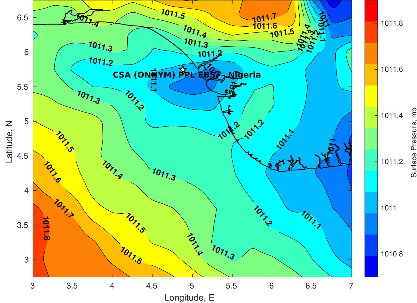
Surface Pressure (mb) for CSA (ONHYM) PPL EBS - Nigeria at 18-Nov-2025 00:00:00
