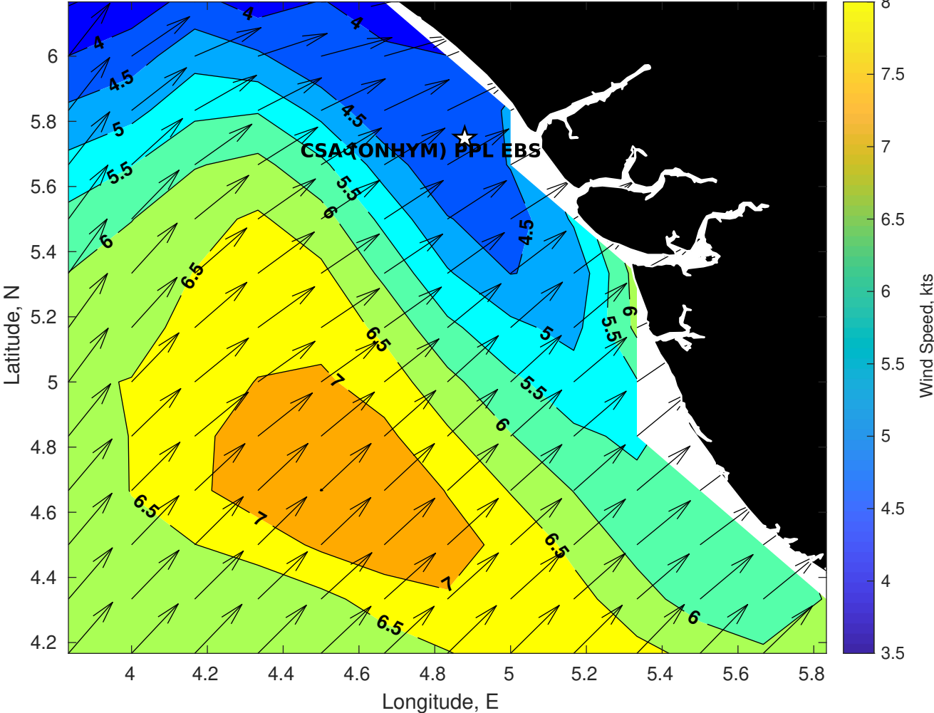
Winds (kts) for CSA (ONHYM) PPL EBS - Nigeria at 18-Nov-2025 09:00:00
