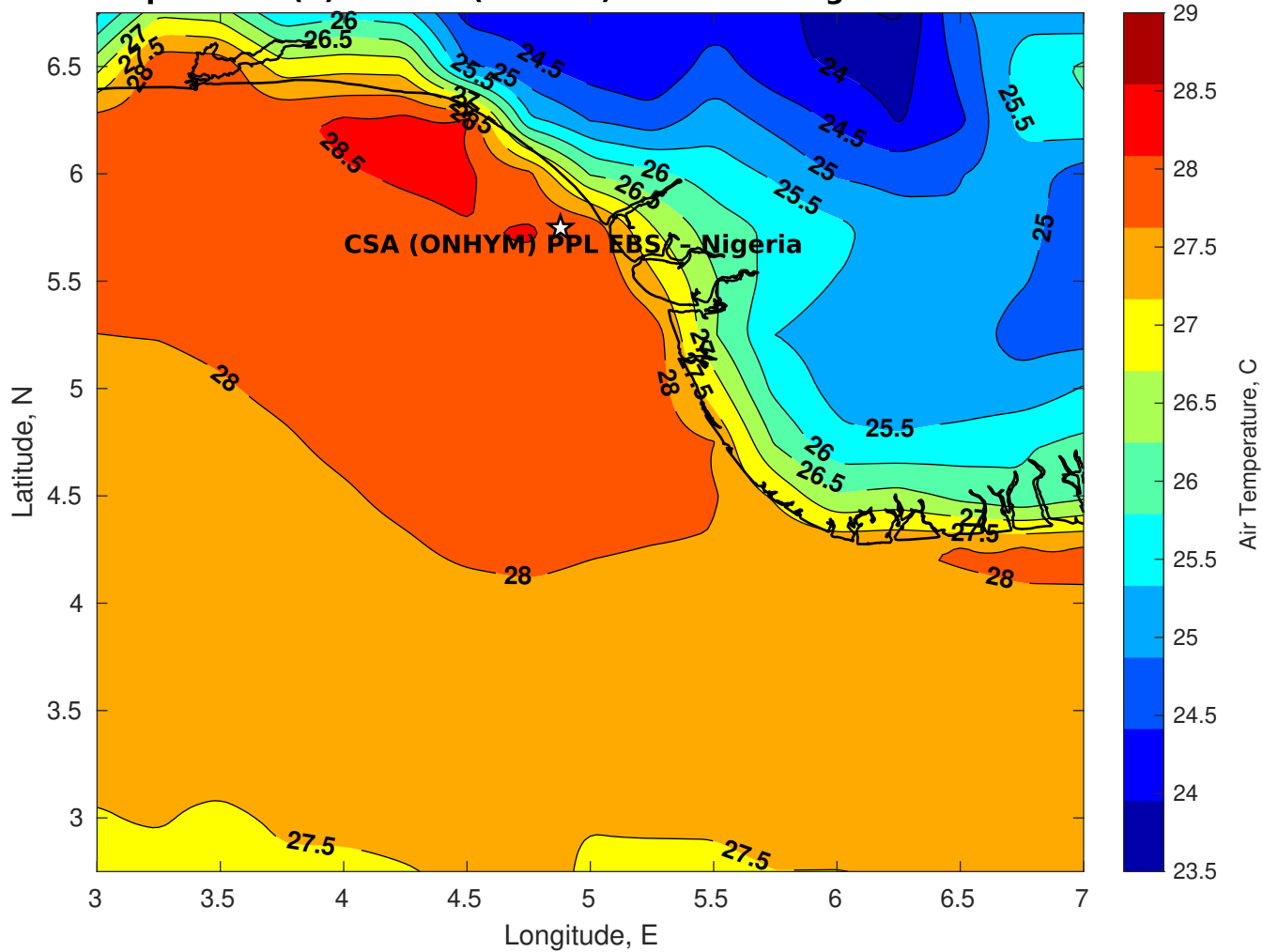
Air Temperature (C) for CSA (ONHYM) PPL EBS - Nigeria at 18-Nov-2025
