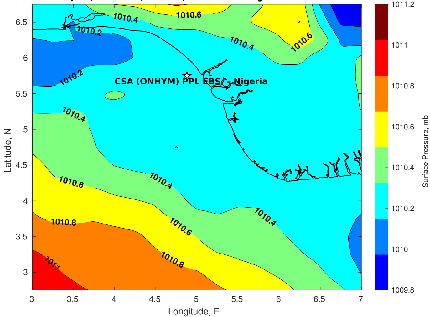
Surface Pressure (mb) for CSA (ONHYM) PPL EBS - Nigeria at 19-Nov-2025 00:00:00
