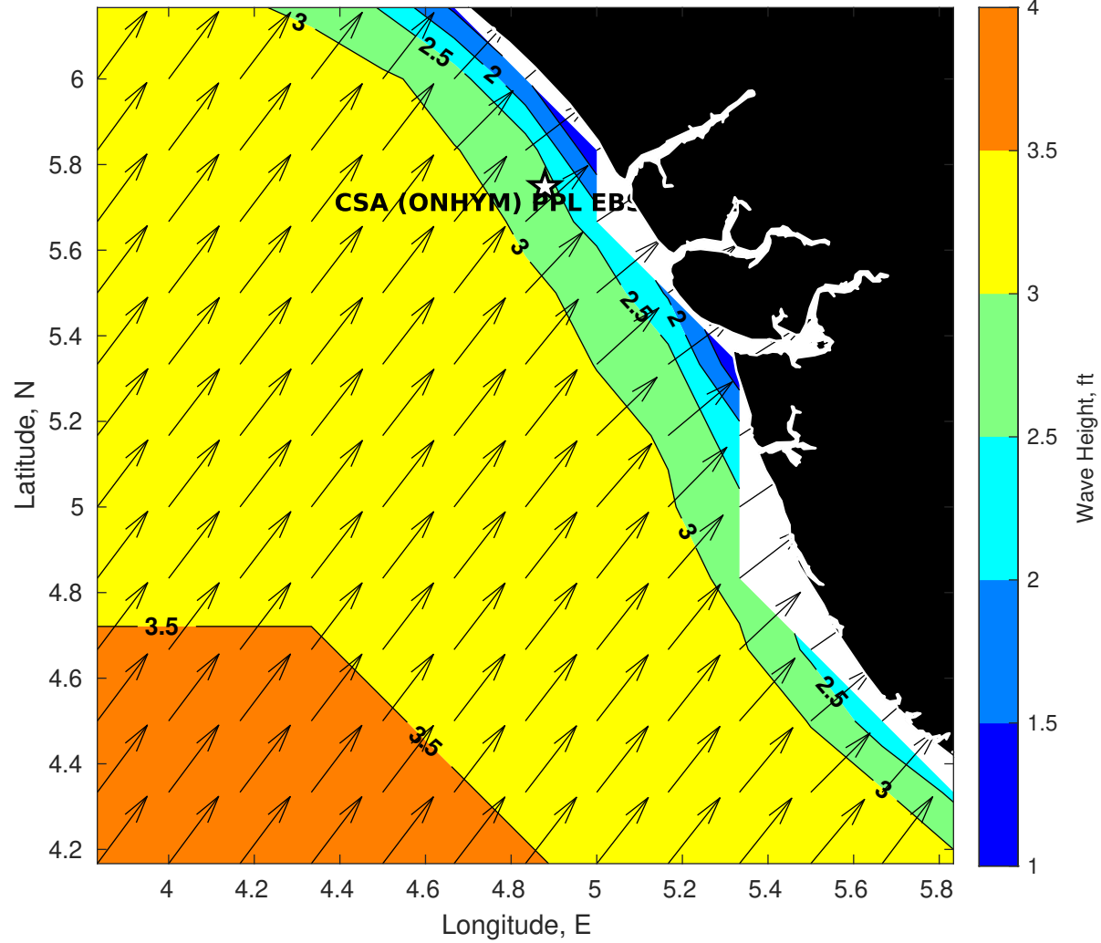
Wave Height (ft) for CSA (ONHYM) PPL EBS - Nigeria at 18-Nov-2025 09:00:00
