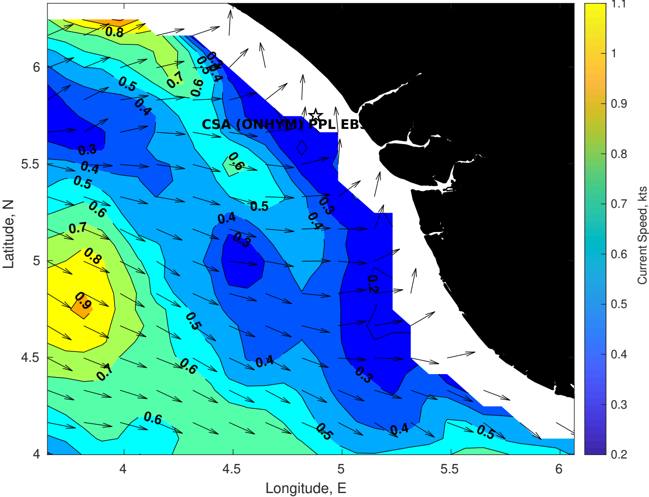
Surface Currents for CSA (ONHYM) PPL EBS - Nigeria at 15-Nov-2025 00:00:00
