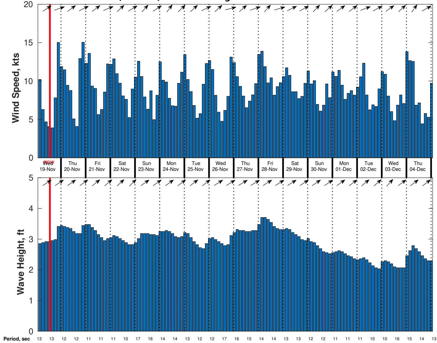
Wind & Wave Forecast for CSA (ONHYM) PPL EBS - Nigeria from 18-Nov-2025 02:00:00 to 04-Dec-2025 02:00:00
