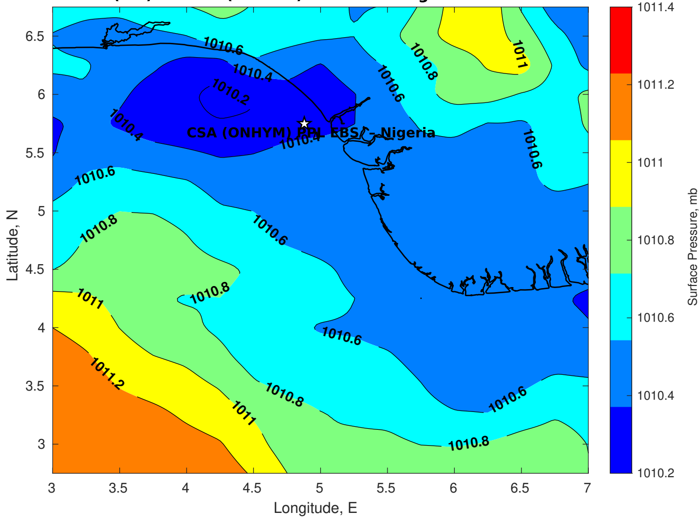
Surface Pressure (mb) for CSA (ONHYM) PPL EBS - Nigeria at 20-Nov-2025 00:00:00
