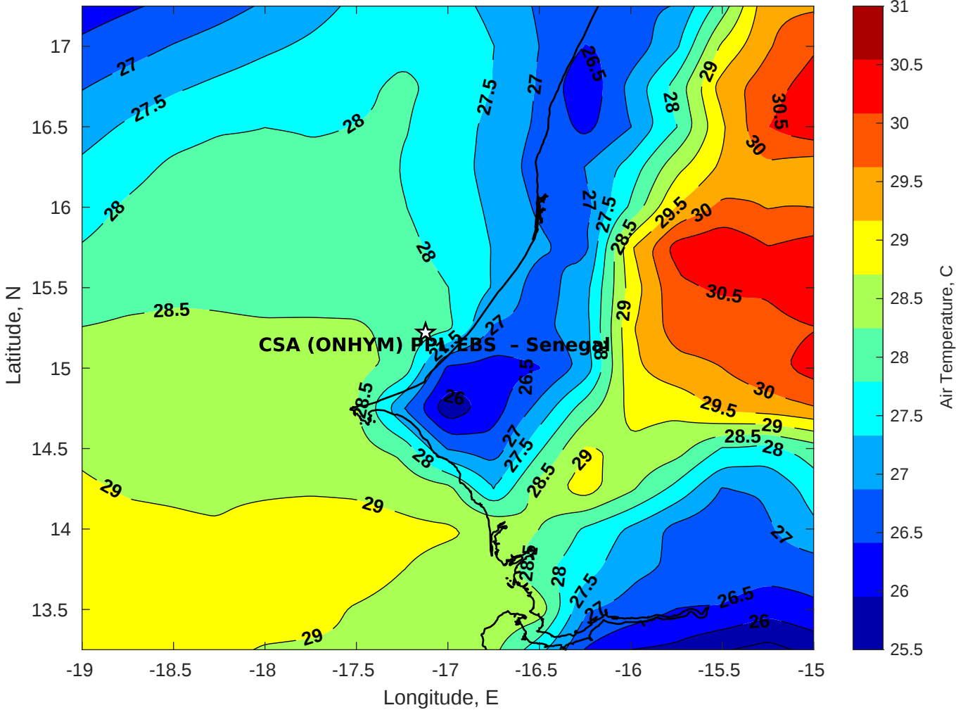
Air Temperature (C) for CSA (ONHYM) PPL EBS - Senegal at 18-Nov-2025
