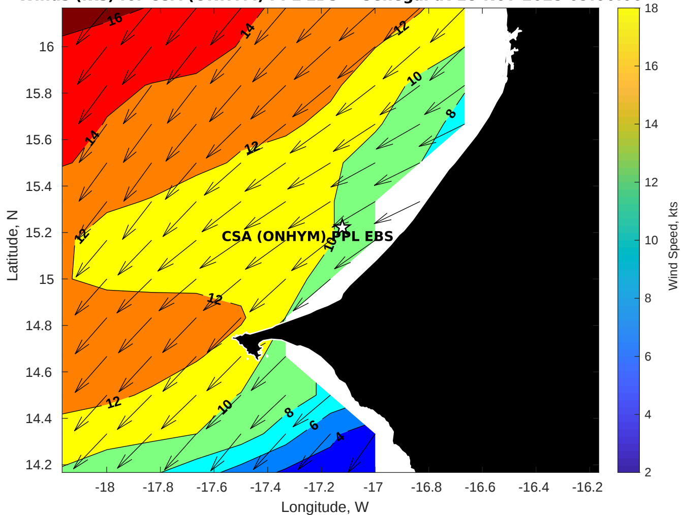
Winds (kts) for CSA (ONHYM) PPL EBS - Senegal at 18-Nov-2025 09:00:00
