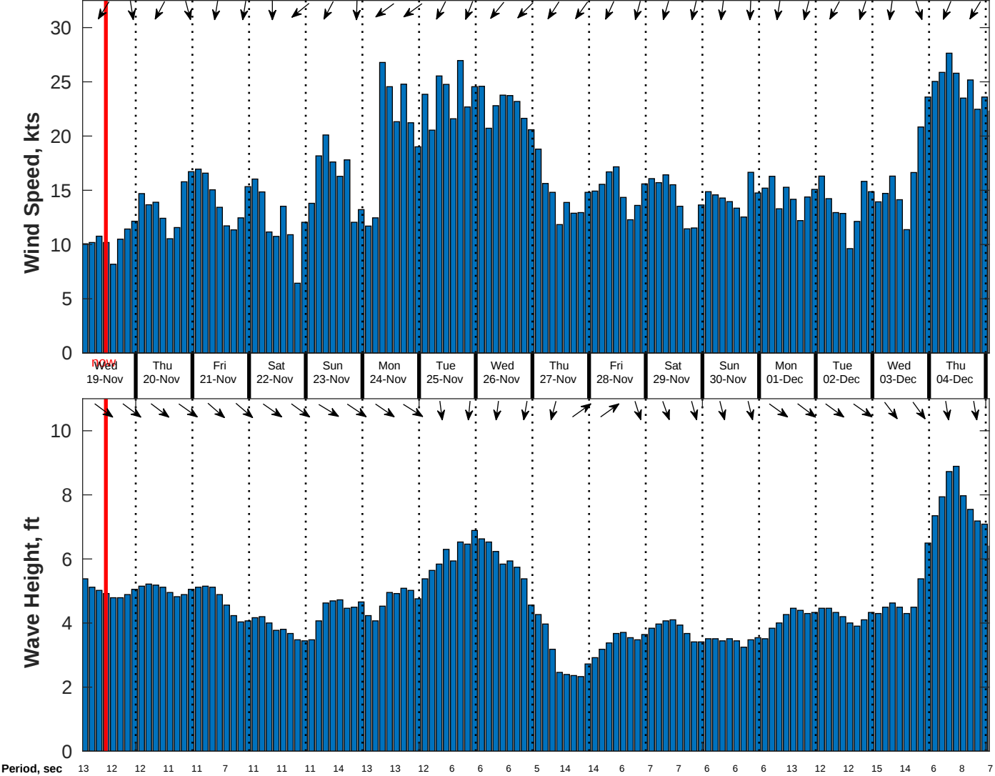
Wind & Wave Forecast for CSA (ONHYM) PPL EBS - Senegal from 18-Nov-2025 01:00:00 to 04-Dec-2025 01:00:00
