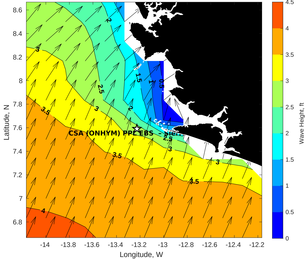
Wave Height (ft) for CSA (ONHYM) PPL EBS - Sierra Leone at 18-Nov-2025 09:00:00
