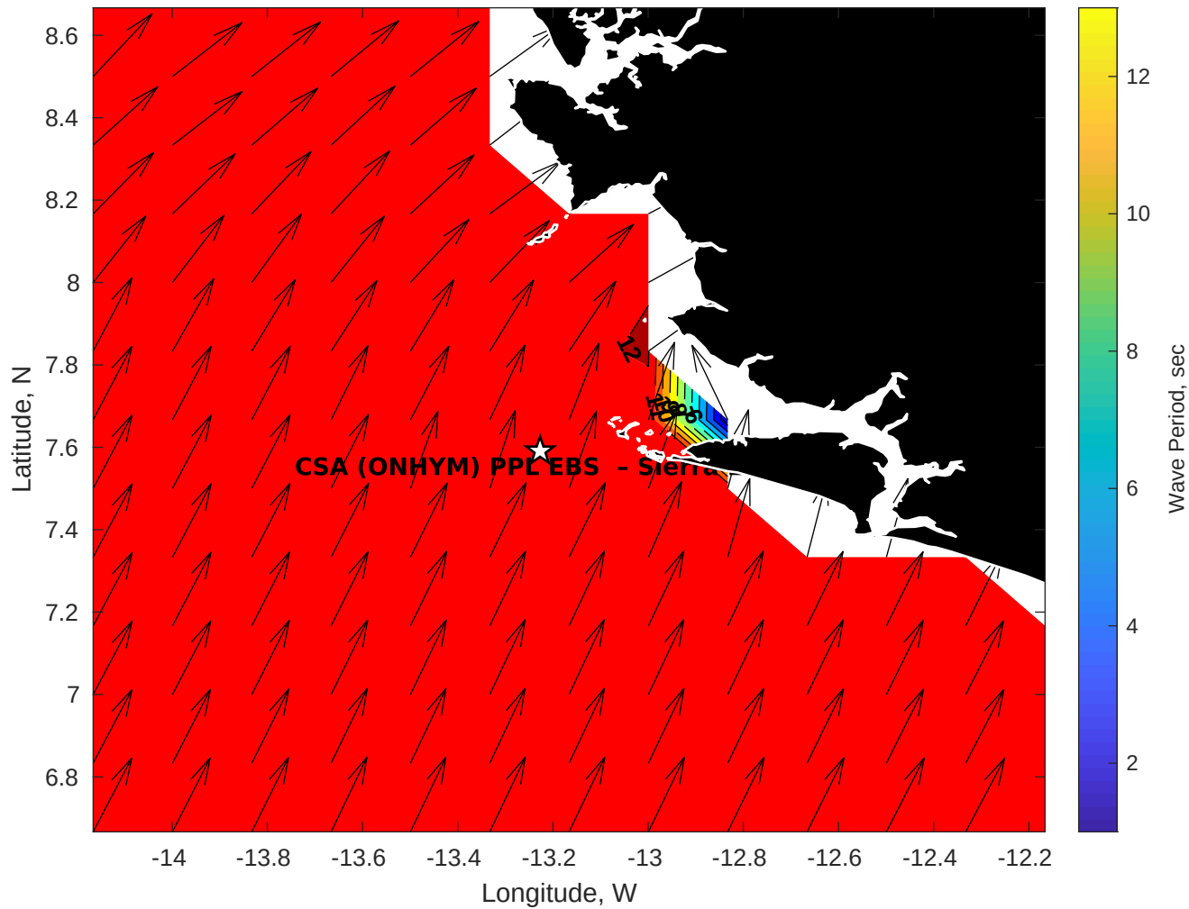
Wave Period (sec) for CSA (ONHYM) PPL EBS - Sierra Leone at 18-Nov-2025 09:00:00
