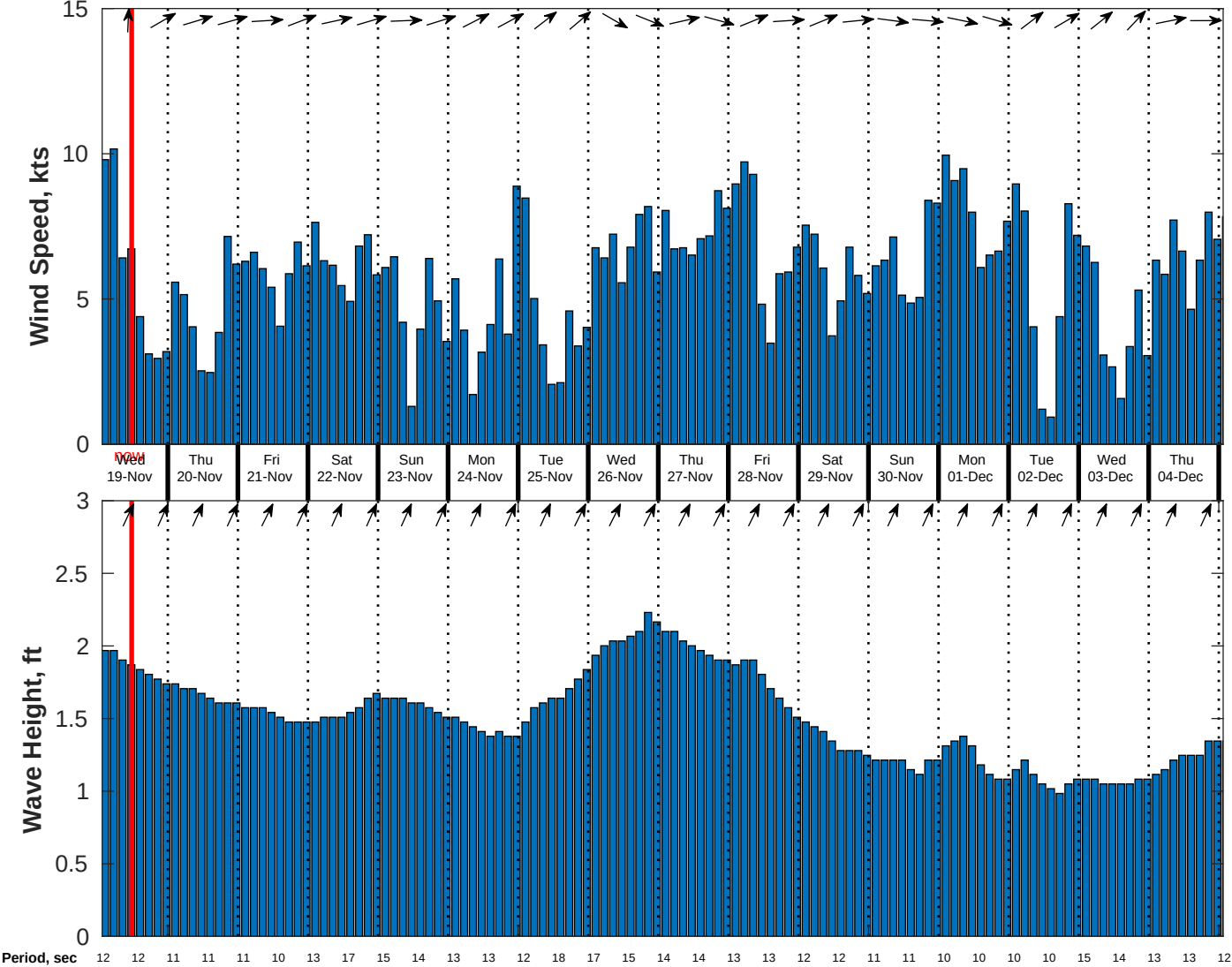
Wind & Wave Forecast for CSA (ONHYM) PPL EBS - Sierra Leone from 18-Nov-2025 01:00:00 to 04-Dec-2025 01:00:00
