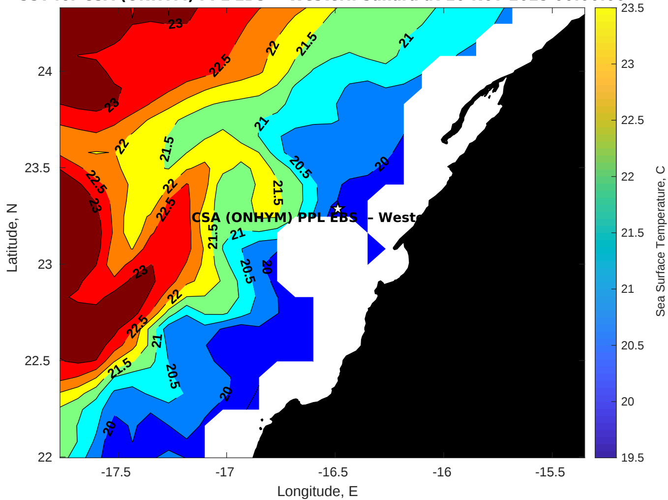
SST for CSA (ONHYM) PPL EBS - Western Sahara at 16-Nov-2025 00:00:00
