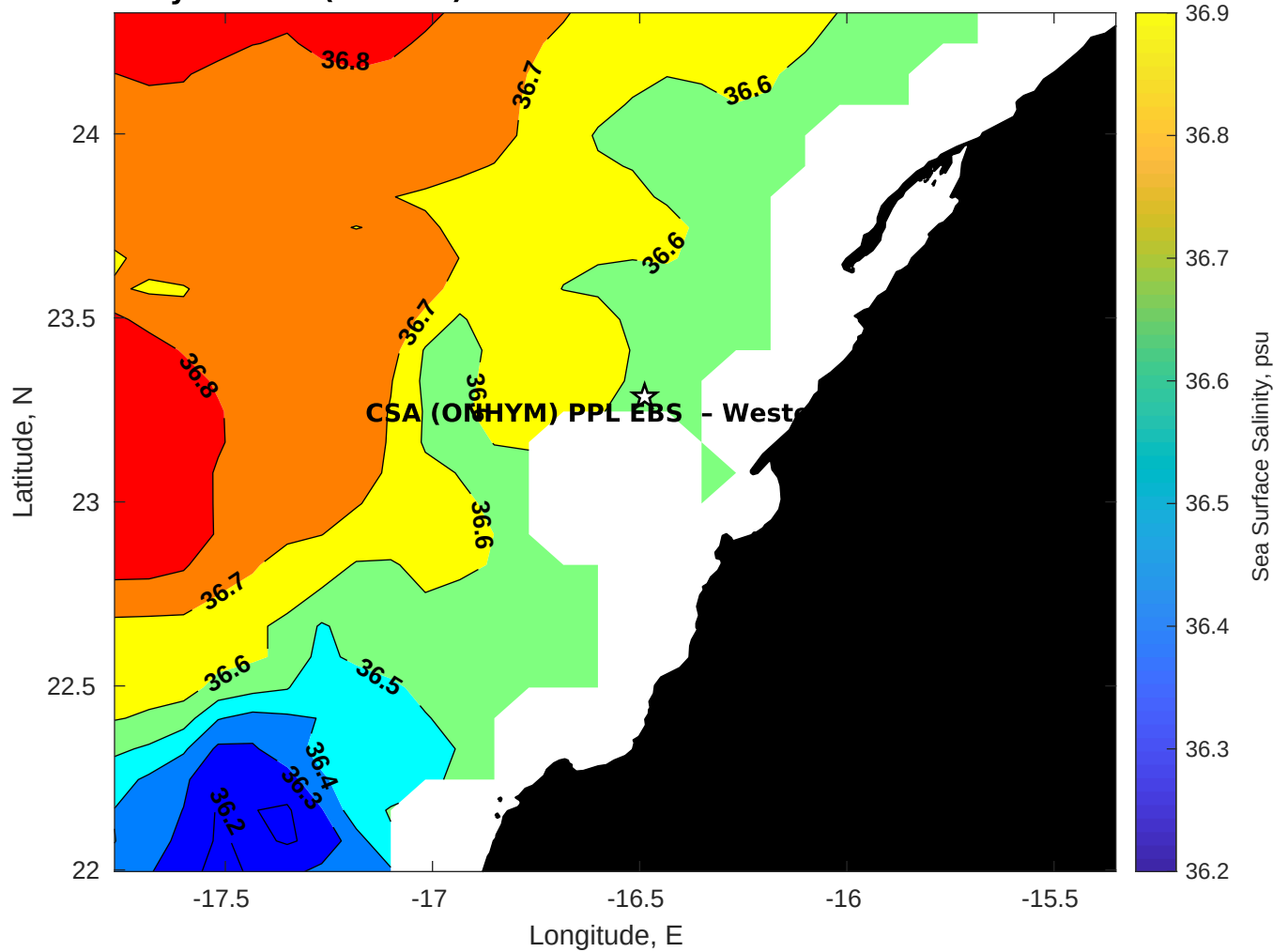
Surface Salinity for CSA (ONHYM) PPL EBS - Western Sahara at 16-Nov-2025 00:00:00
