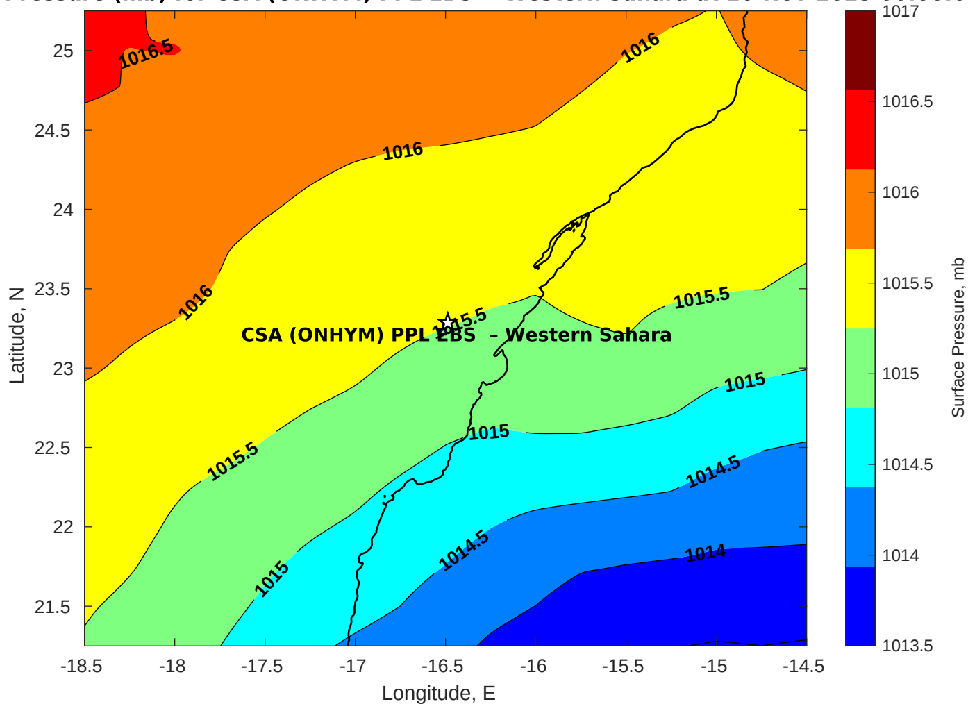
Surface Pressure (mb) for CSA (ONHYM) PPL EBS - Western Sahara at 20-Nov-2025 00:00:00
