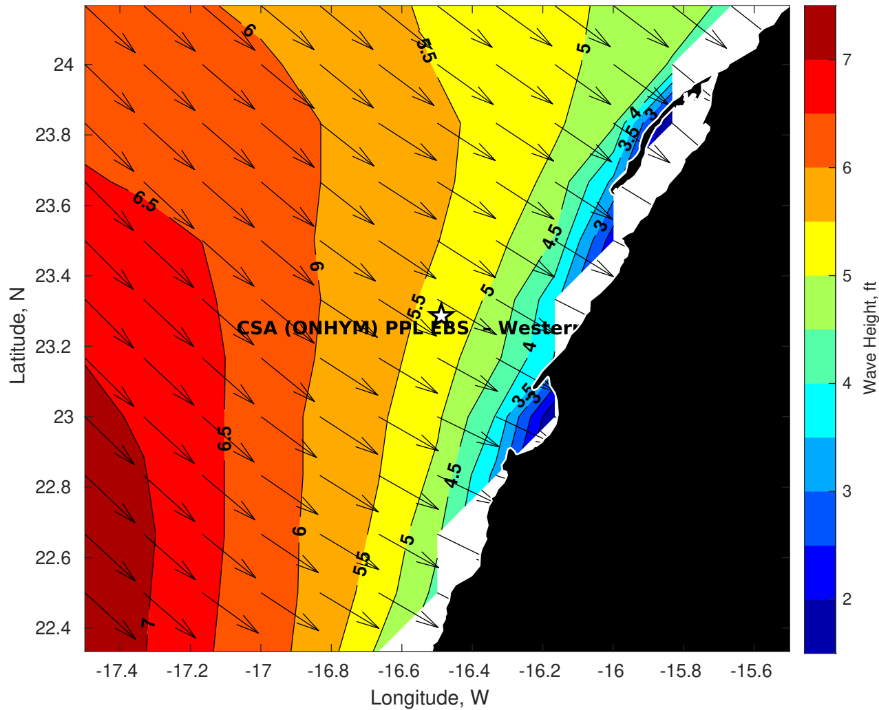
Wave Height (ft) for CSA (ONHYM) PPL EBS - Western Sahara at 18-Nov-2025 09:00:00
