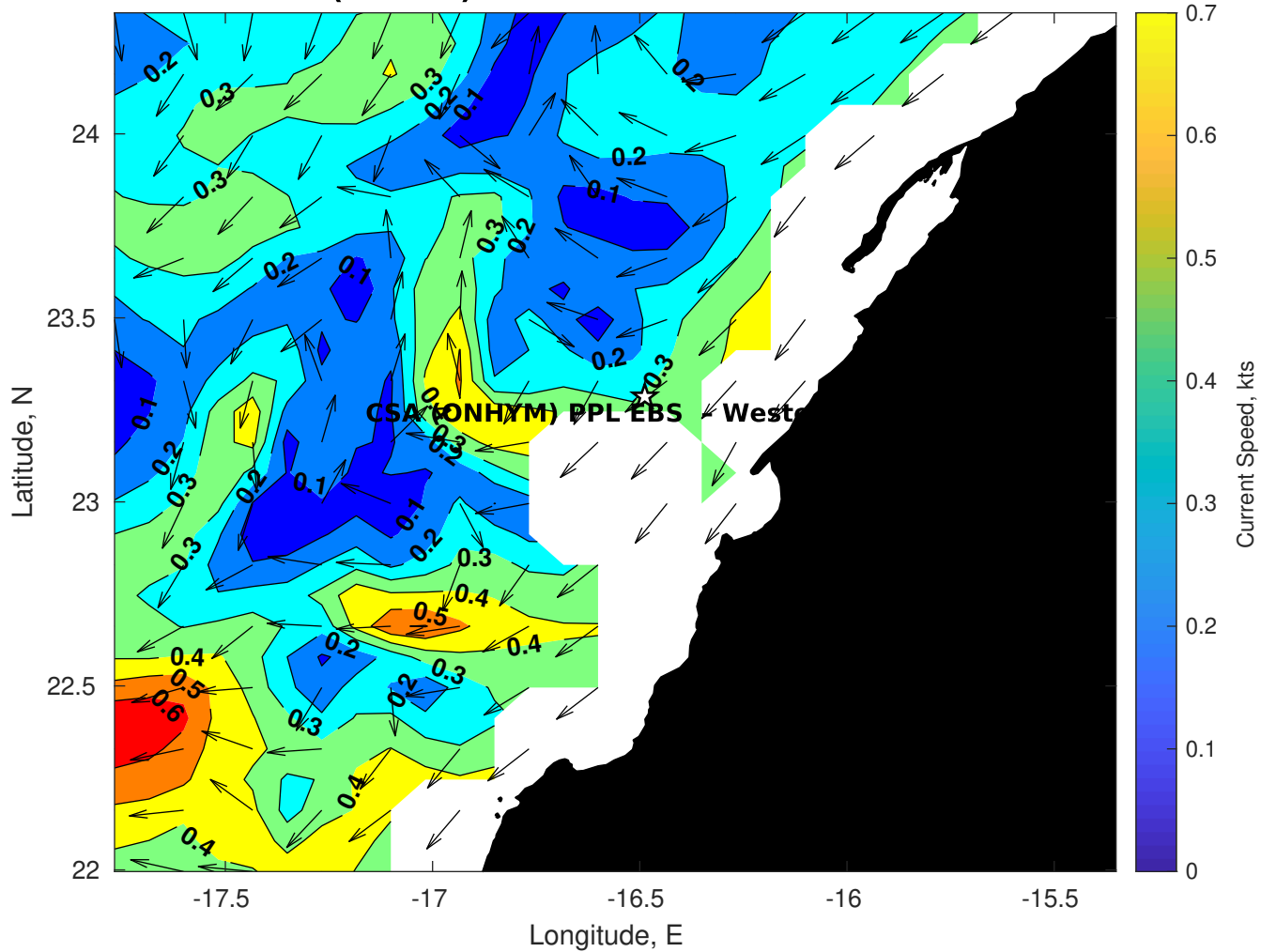
Surface Currents for CSA (ONHYM) PPL EBS - Western Sahara at 16-Nov-2025 00:00:00
