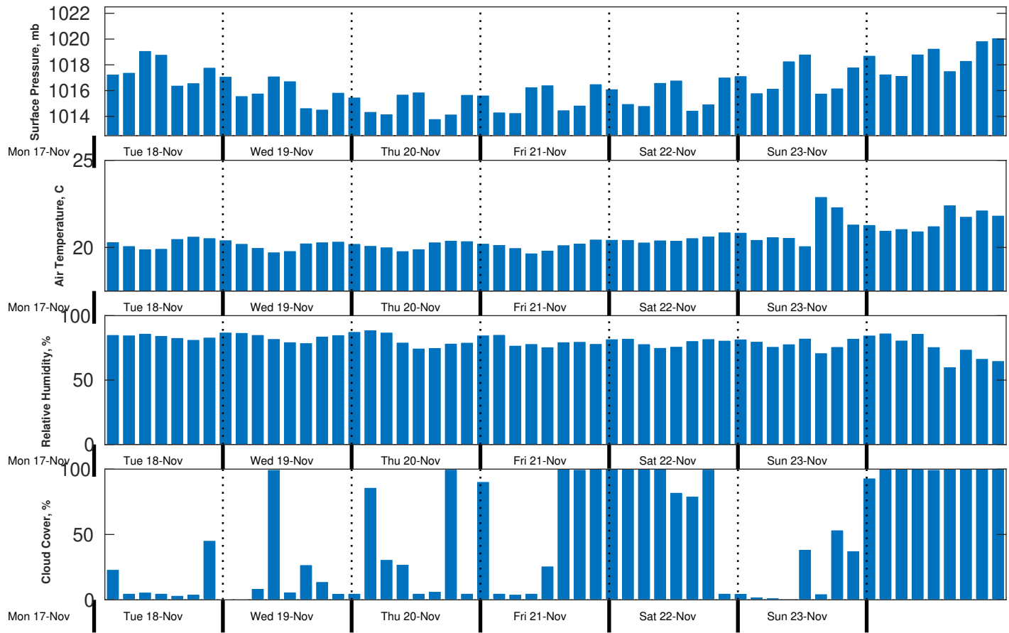
Met Forecast for CSA (ONHYM) PPL EBS - Western Sahara from 18-Nov-2025 00:00:00 to 25-Nov-2025 00:00:00
