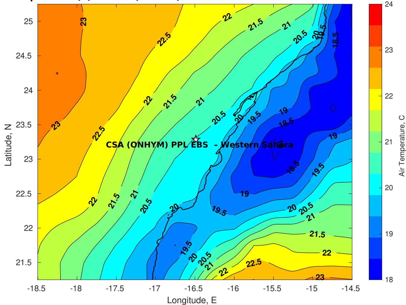
Air Temperature (C) for CSA (ONHYM) PPL EBS - Western Sahara at 18-Nov-2025
