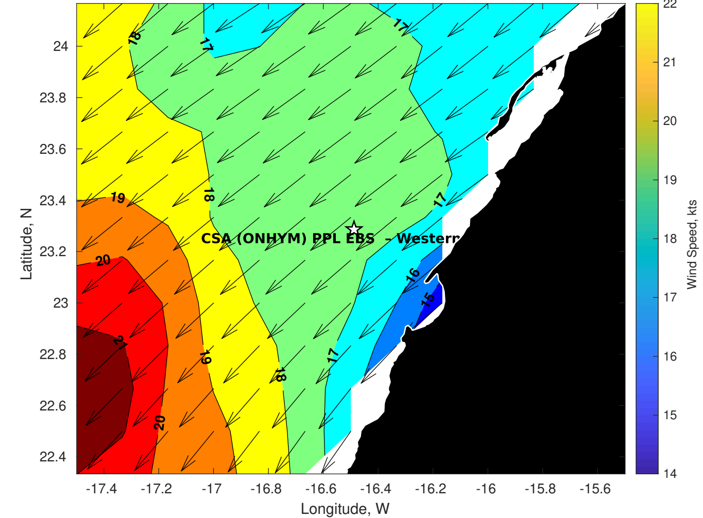
Winds (kts) for CSA (ONHYM) PPL EBS - Western Sahara at 18-Nov-2025 09:00:00
