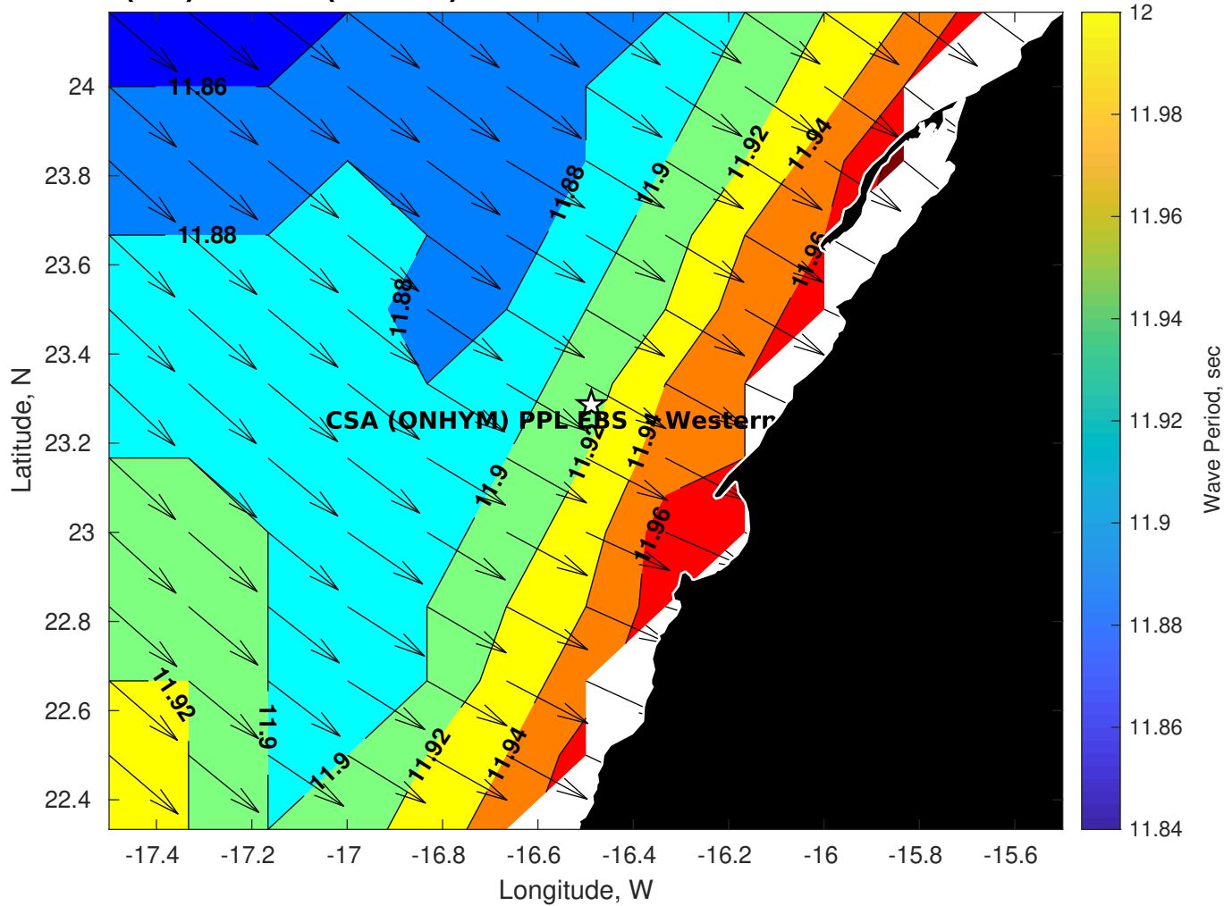
Wave Period (sec) for CSA (ONHYM) PPL EBS - Western Sahara at 18-Nov-2025 09:00:00
