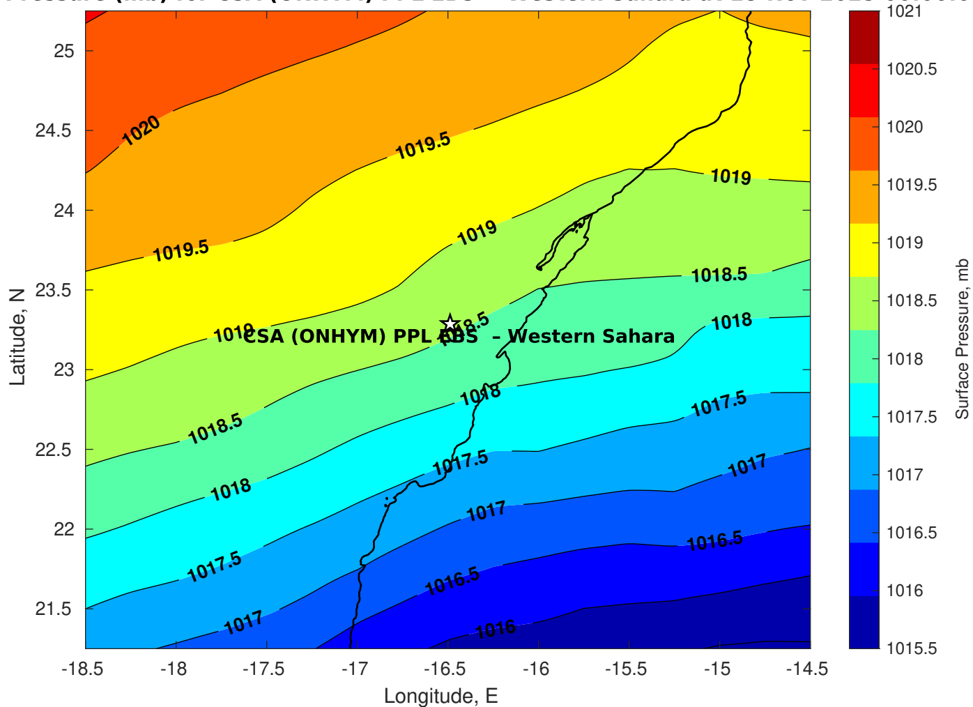
Surface Pressure (mb) for CSA (ONHYM) PPL EBS - Western Sahara at 18-Nov-2025 00:00:00
