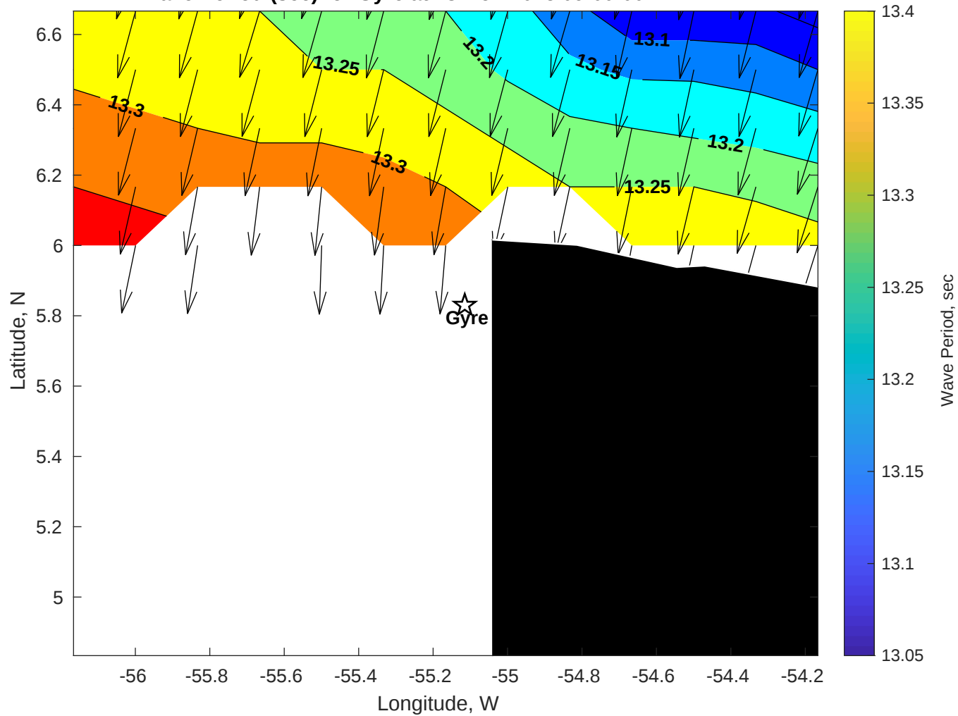
Wave Period (sec) for Gyre at 18-Nov-2025 09:00:00
