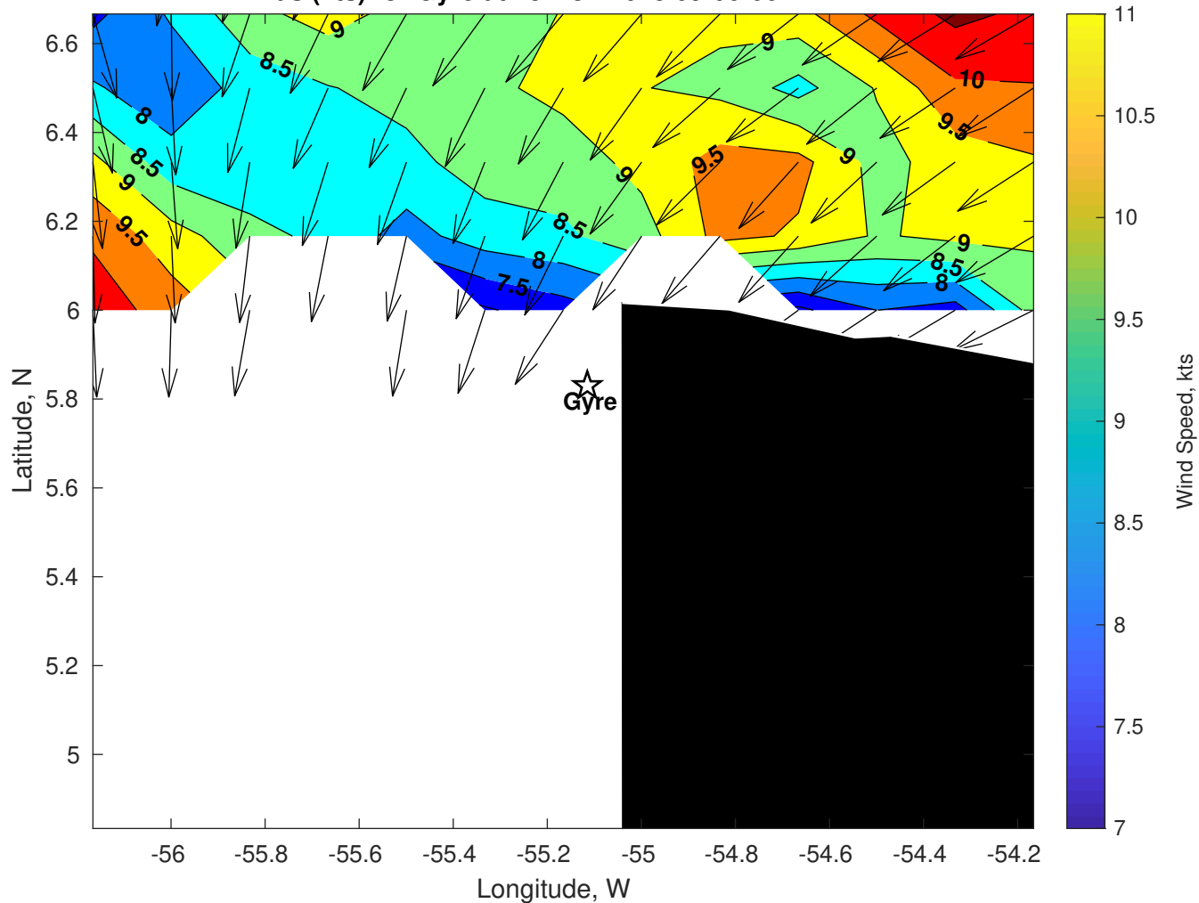
Winds (kts) for Gyre at 18-Nov-2025 09:00:00
