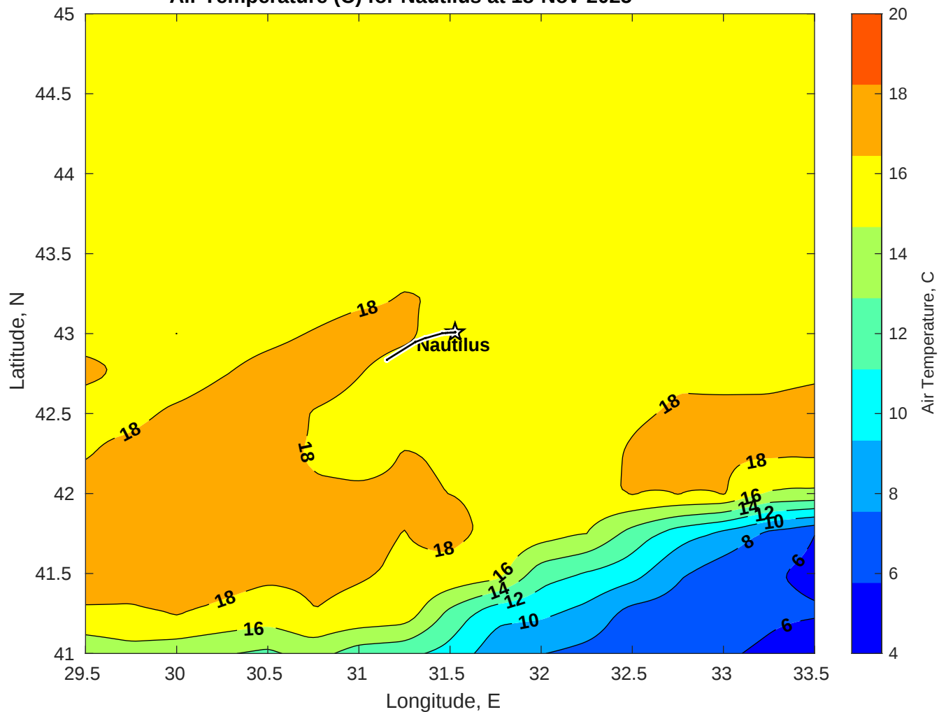
Air Temperature (C) for Nautilus at 18-Nov-2025
